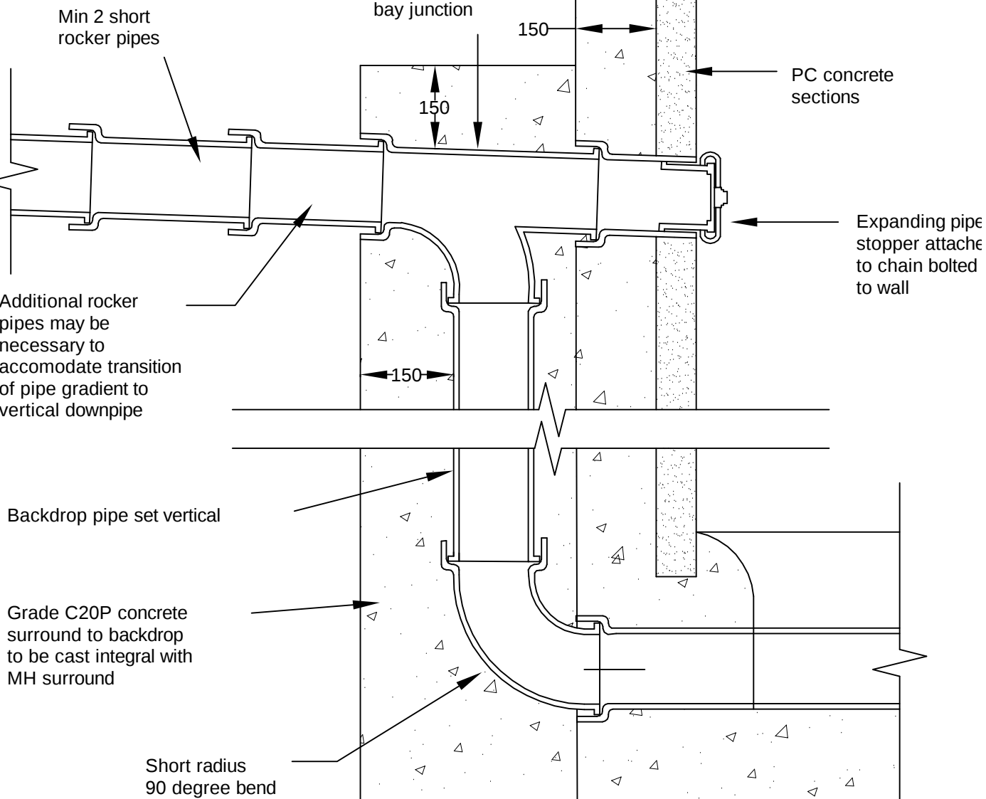
Typical Backdrop Detail. Scale 1:10
