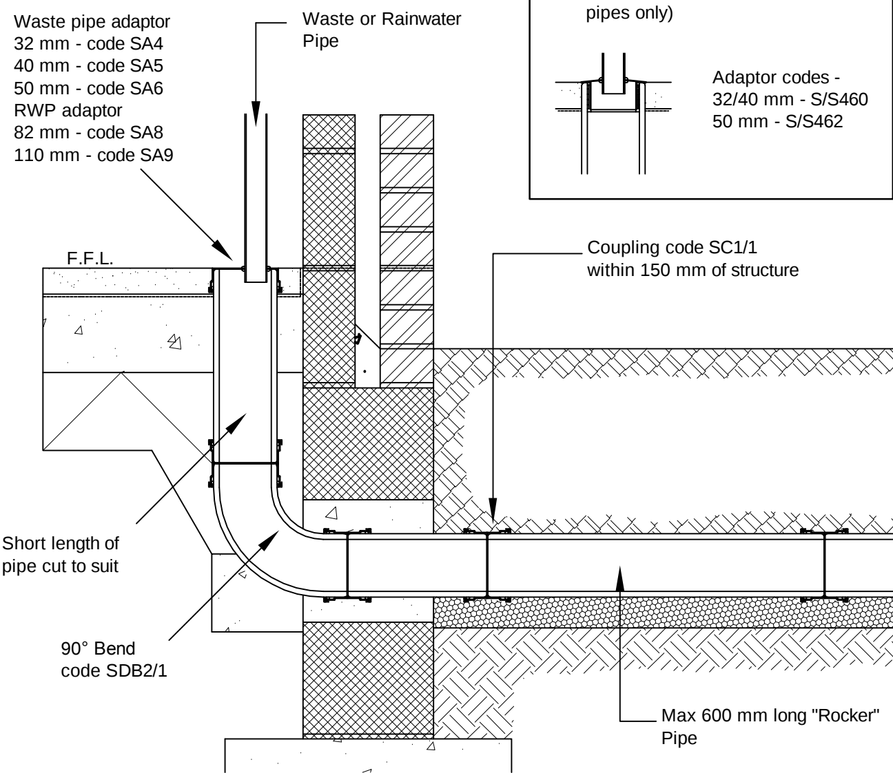
Typical Internal Waste Pipe. Connection Detail DC1 Scale 1:10
