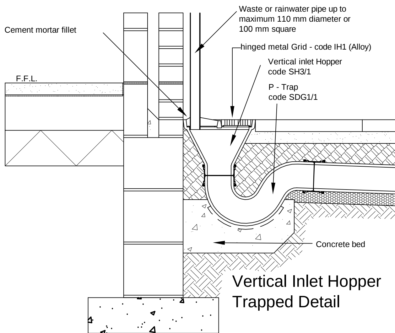
Polypropylene Inspection Chamber Installation Detail. Scale 1:10
