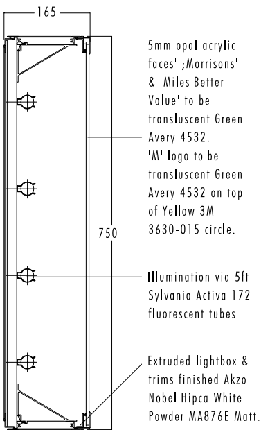
KIOSK scale 1:10 TYPICAL SECTION THROUGH LIGHTBOX ASSEMBLY
