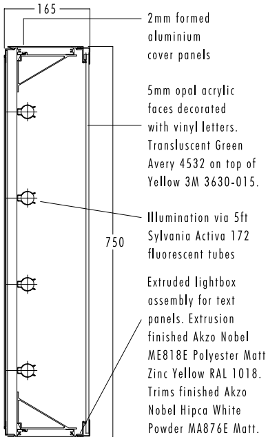
CAR WASH scale 1:10 TYPICAL SECTION THROUGH LIGHTBOX ASSEMBLY
