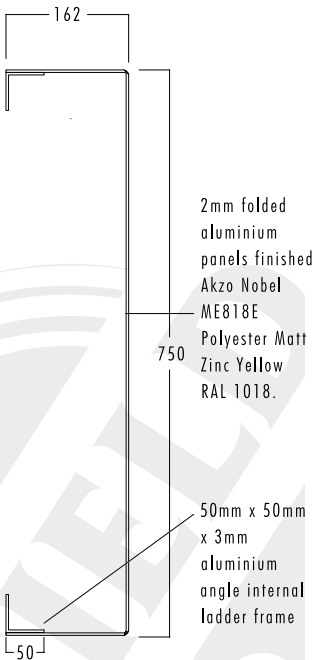
CAR WASH scale 1:10 TYPICAL SECTION THROUGH SIDE PANELS
