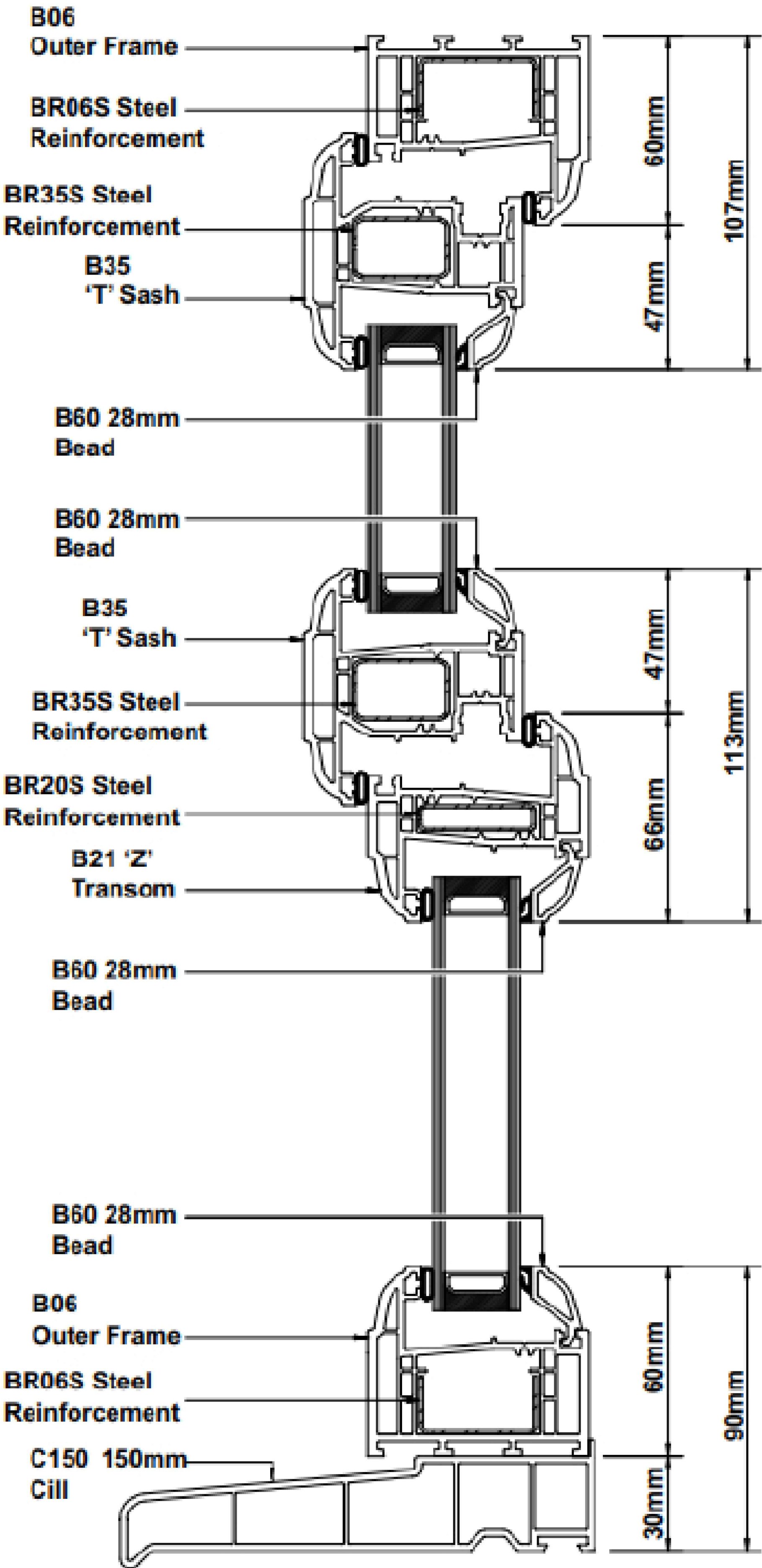
W1 Vertical Section (1:1)
