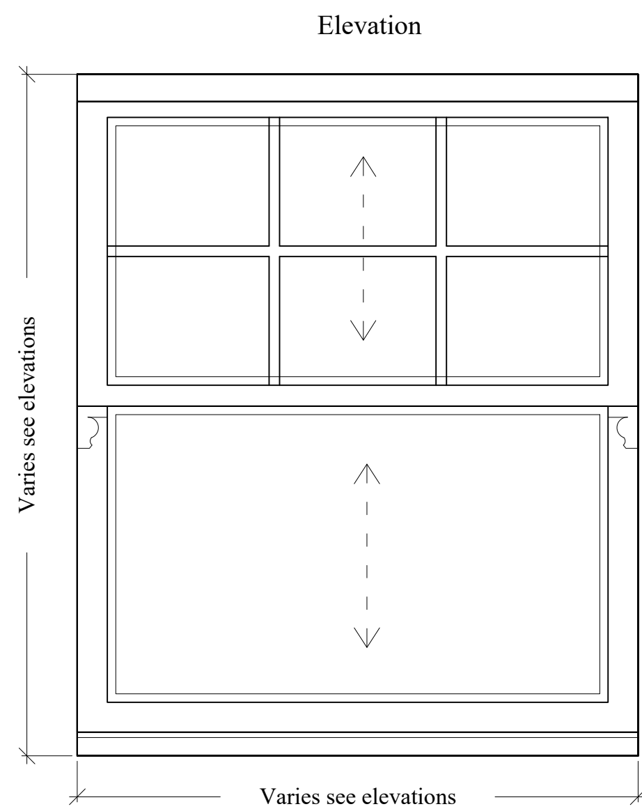
W2, W3 and W4 - Window Detail (1:10)
