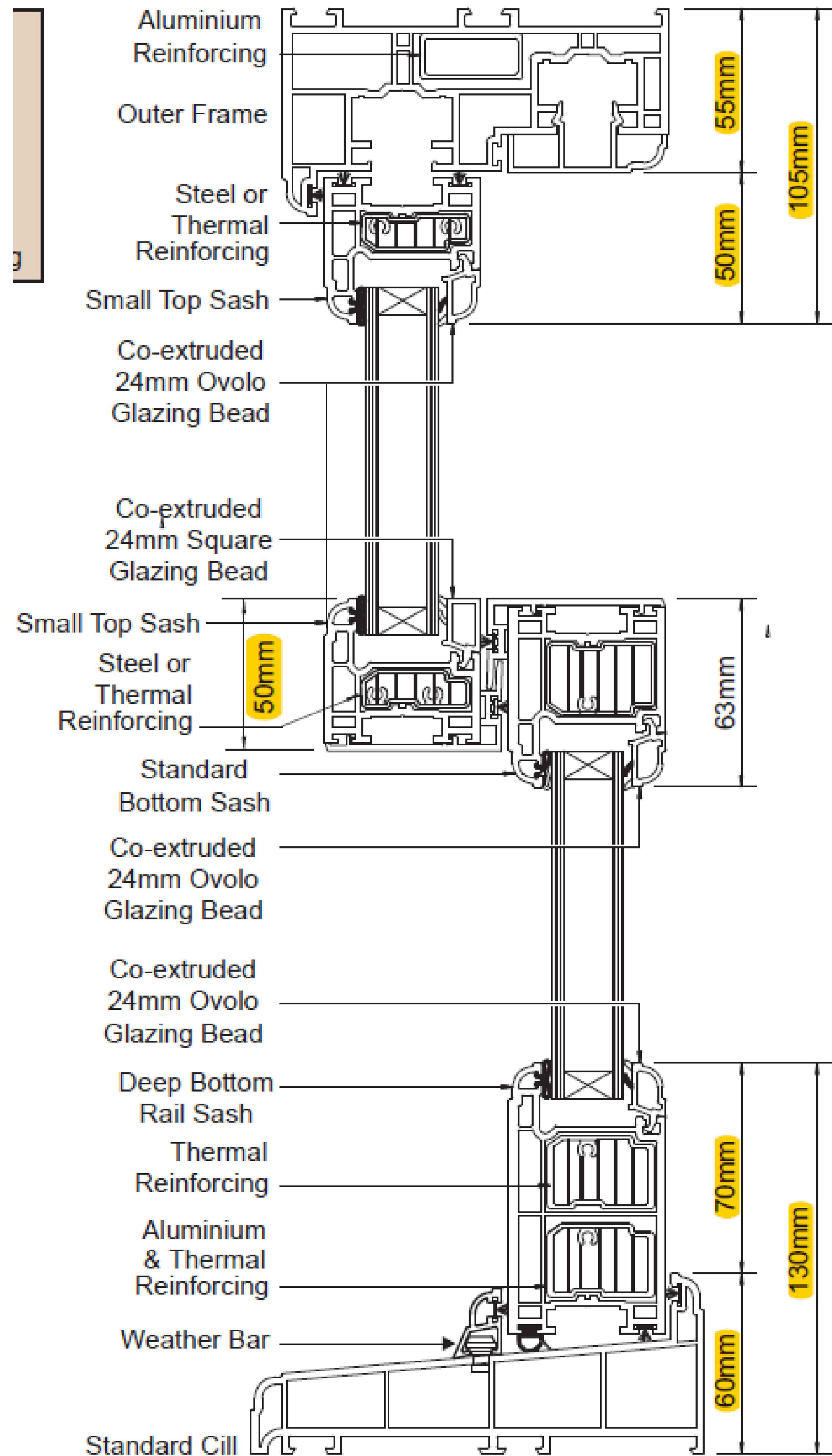
W1 Vertical Section (1:1)
