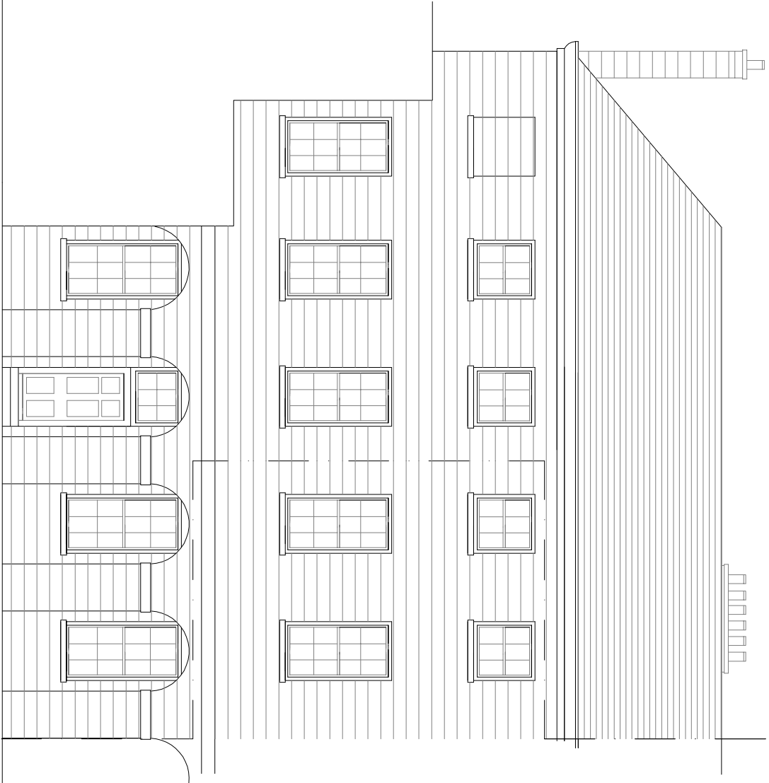
Proposed front elevation - unchanged
