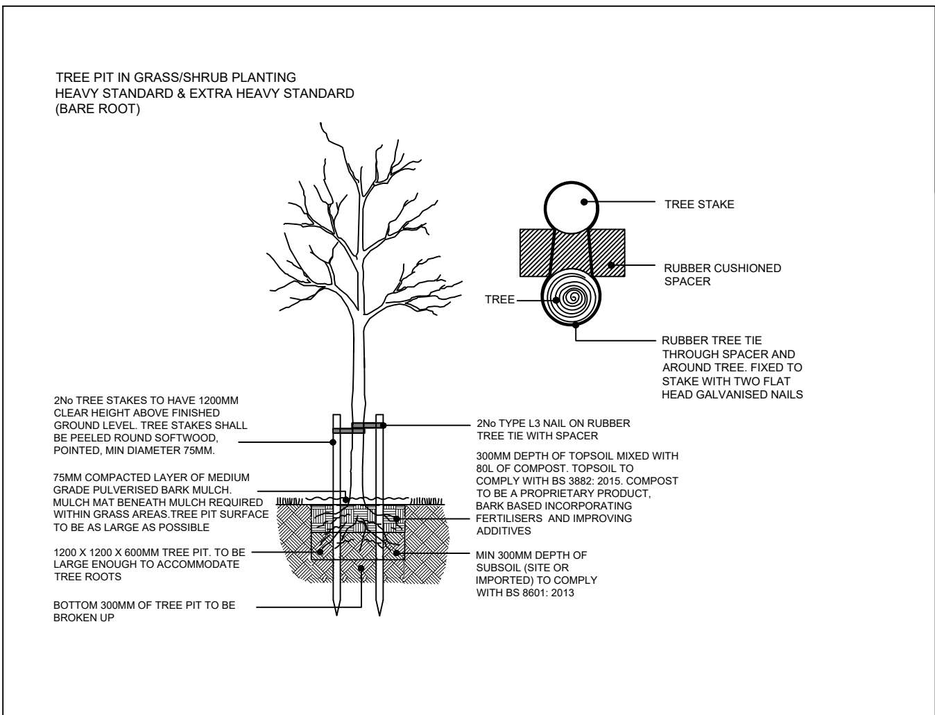
PROPOSED EXTRA HEAVY STANDARD TREE (BARE ROOT) REFER TO PLANT SCHEDULE
