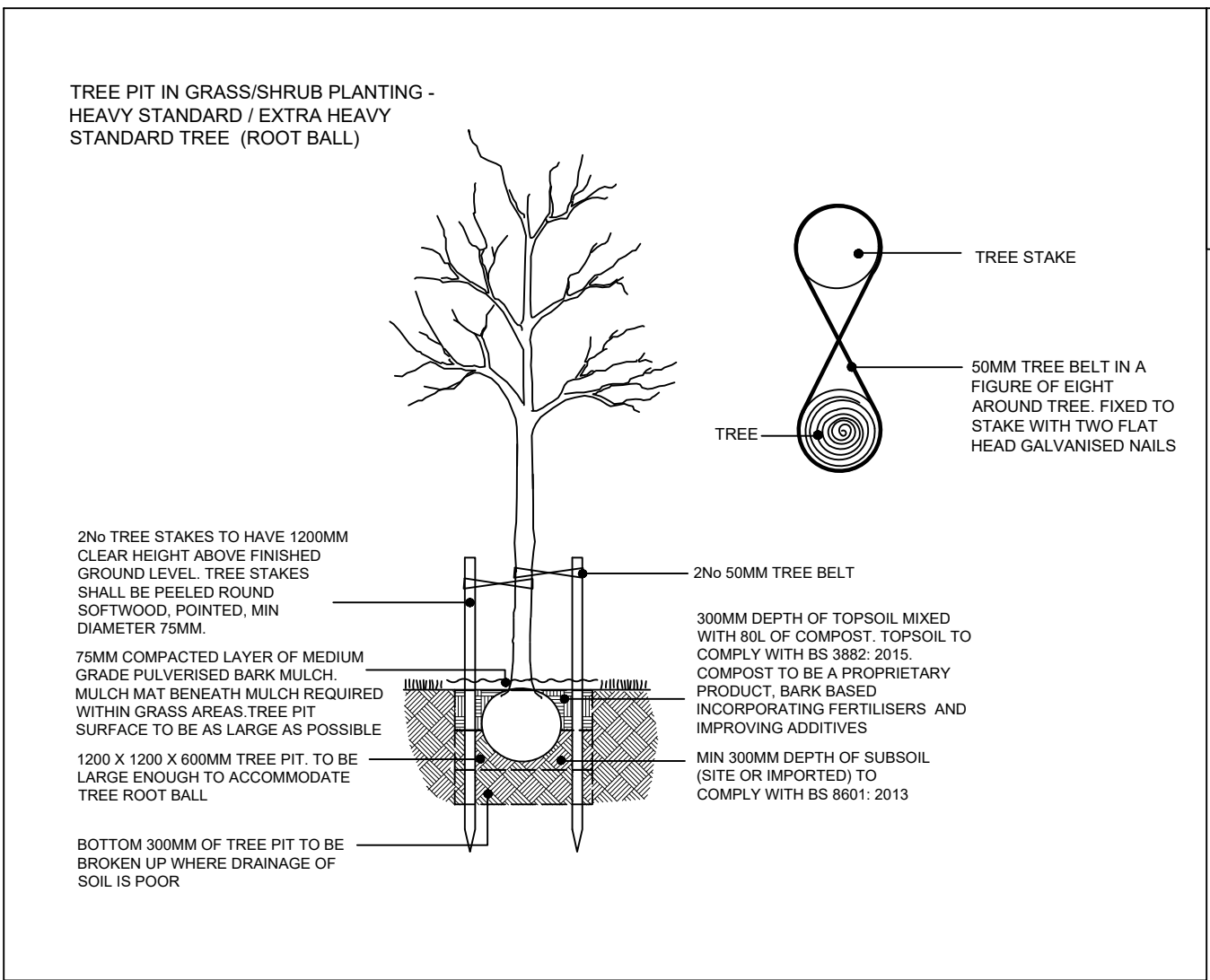
PROPOSED EXTRA HEAVY STANDARD TREE (ROOTBALL) REFER TO PLANT SCHEDULE
