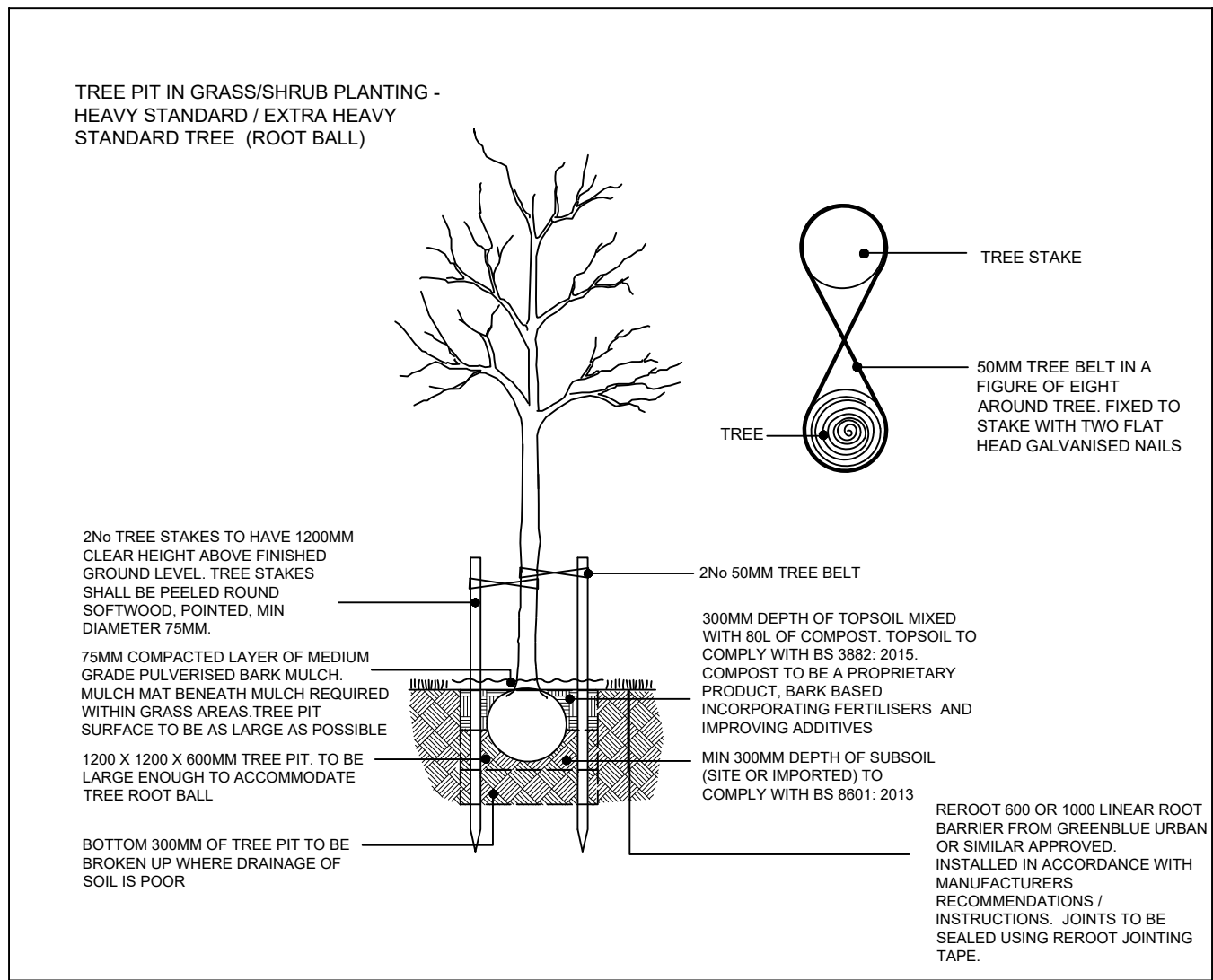
PROPOSED EXTRA HEAVY STANDARD TREE PLANTING WITH ROOT BARRIER REFER TO PLANT SCHEDULE
