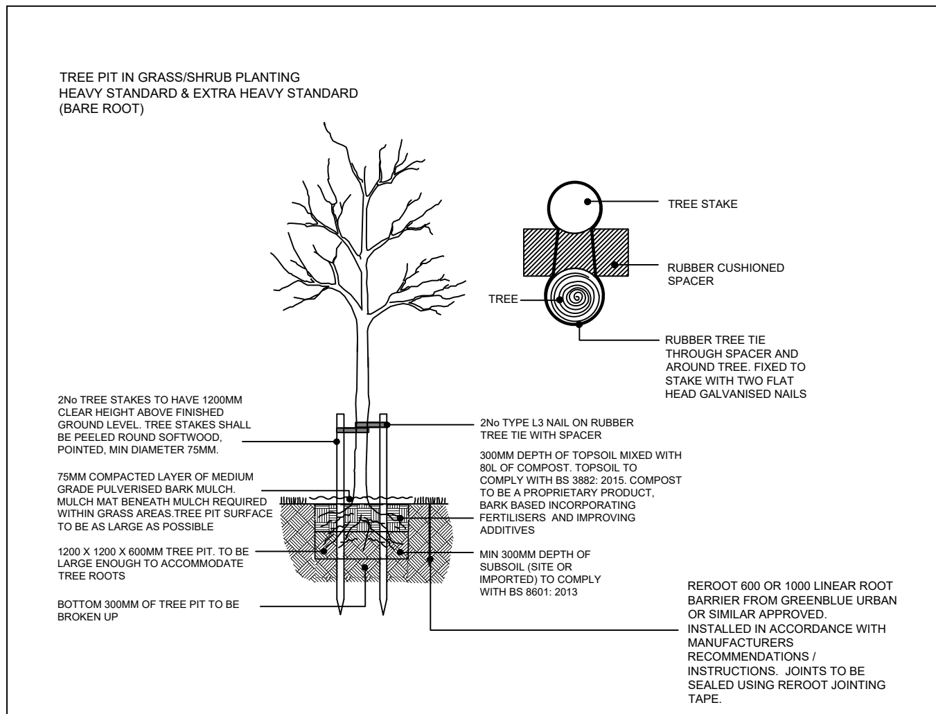
PROPOSED EXTRA HEAVY STANDARD TREE PLANTING WITH ROOT BARRIER REFER TO PLANT SCHEDULE
