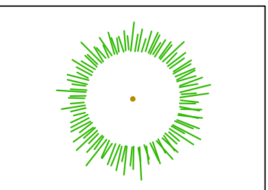
PROPOSED HEAVY STANDARD TREE PLANTING (BARE ROOT) REFER TO PLANT SCHEDULE
