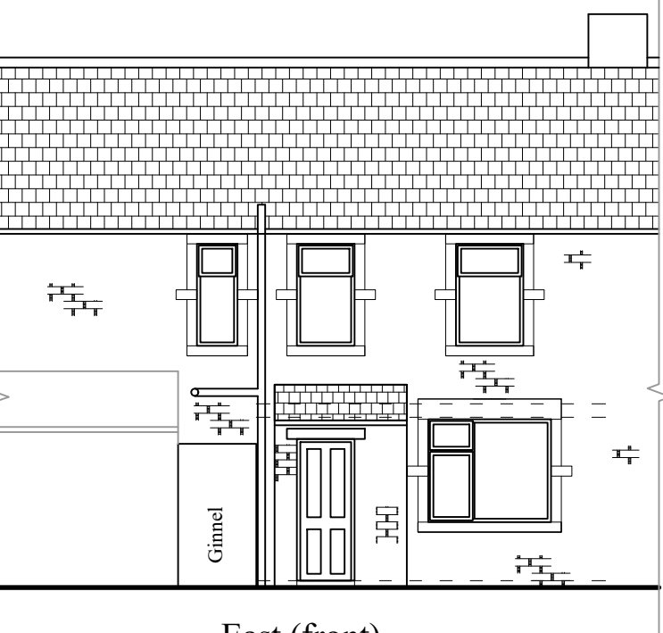
East (front)
