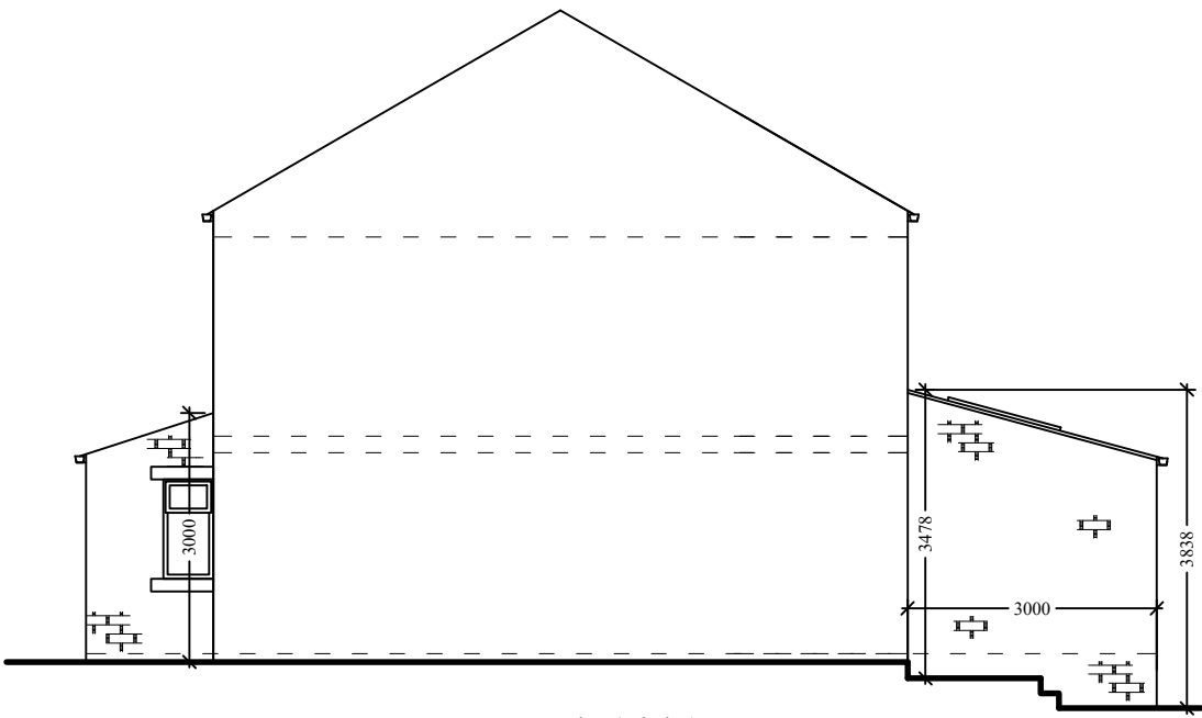
North (side)
