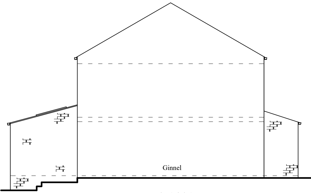
South (side)
