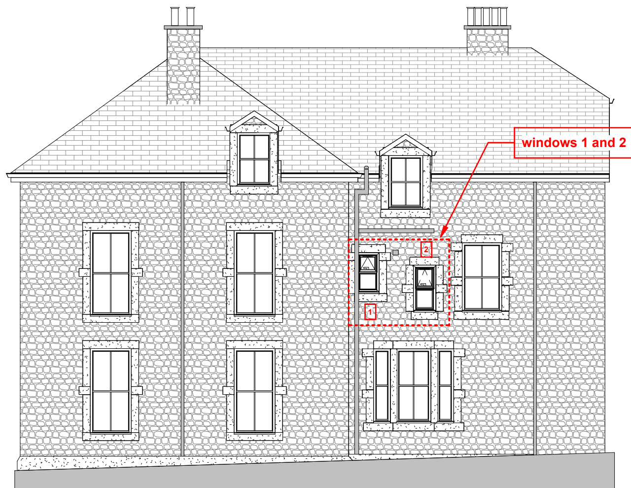
South elevation - existing and proposed
