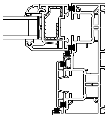
Bottom sash
