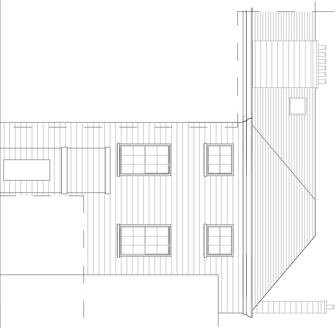
Proposed rear elevation - unchanged
