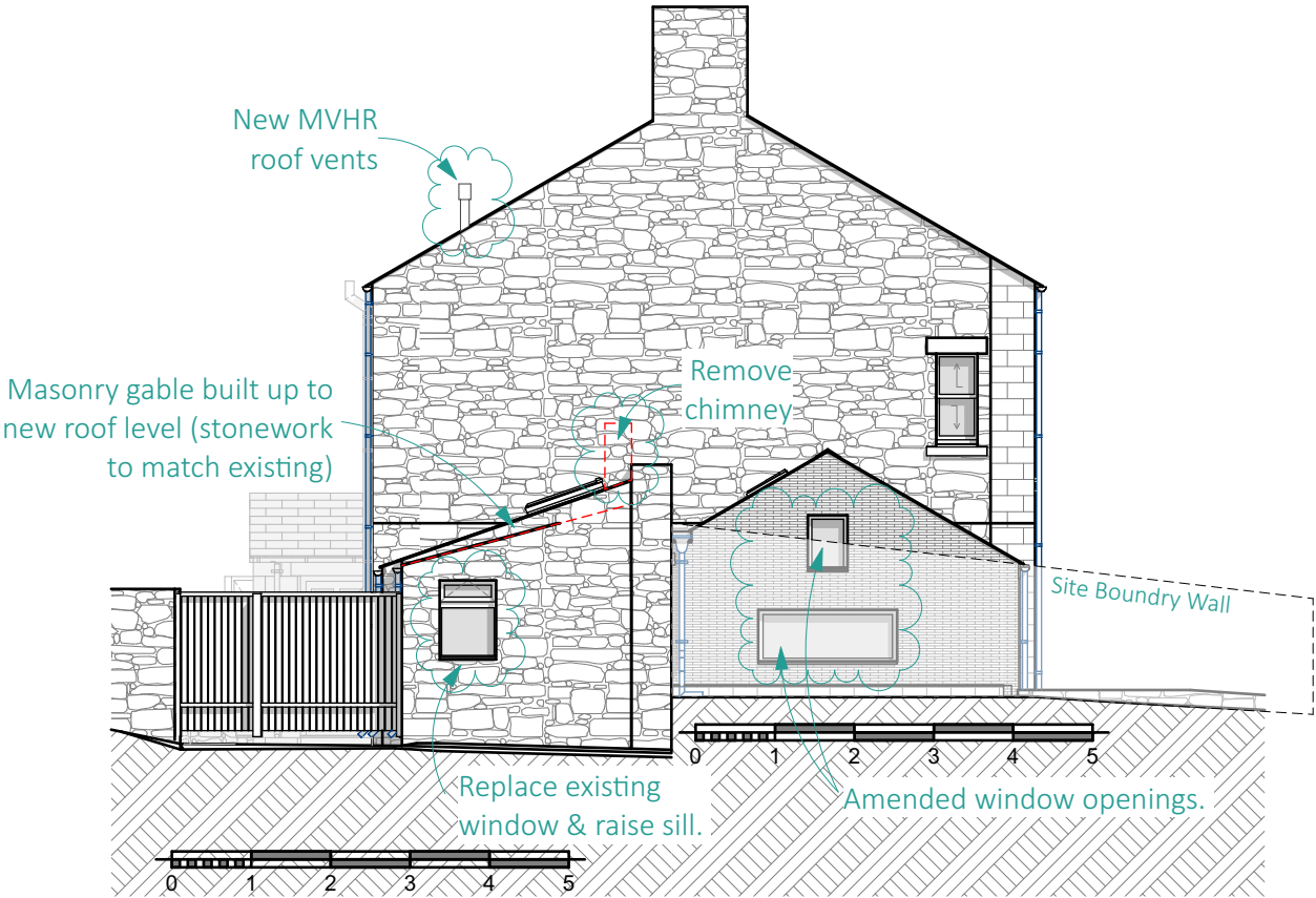
West Elevation | 1:100
