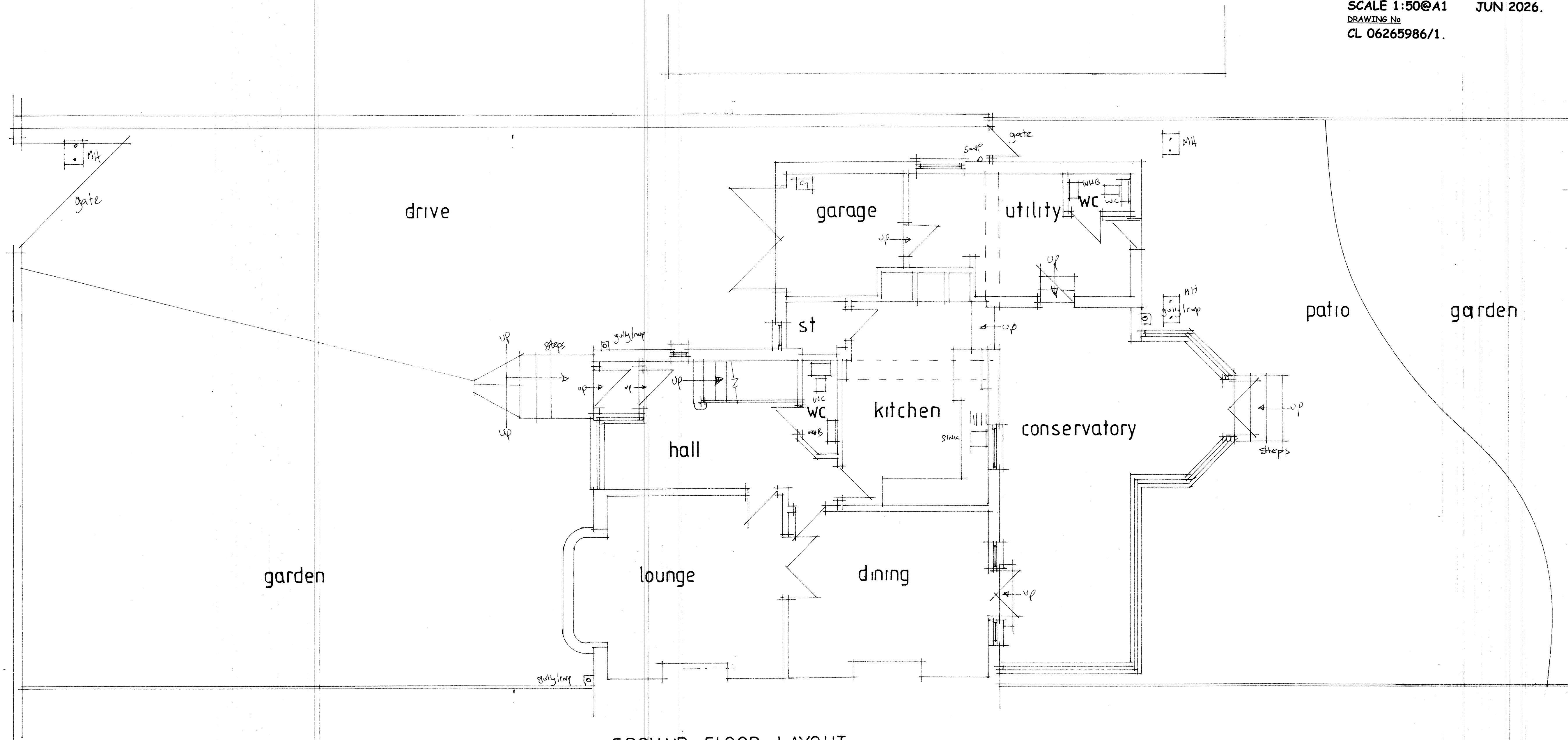
GROUND FLOOR LAYOUT
