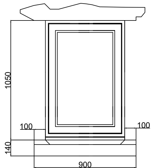
Window: Rear, first floor, right bathroom, obscured glass, Scale 1 / 20
