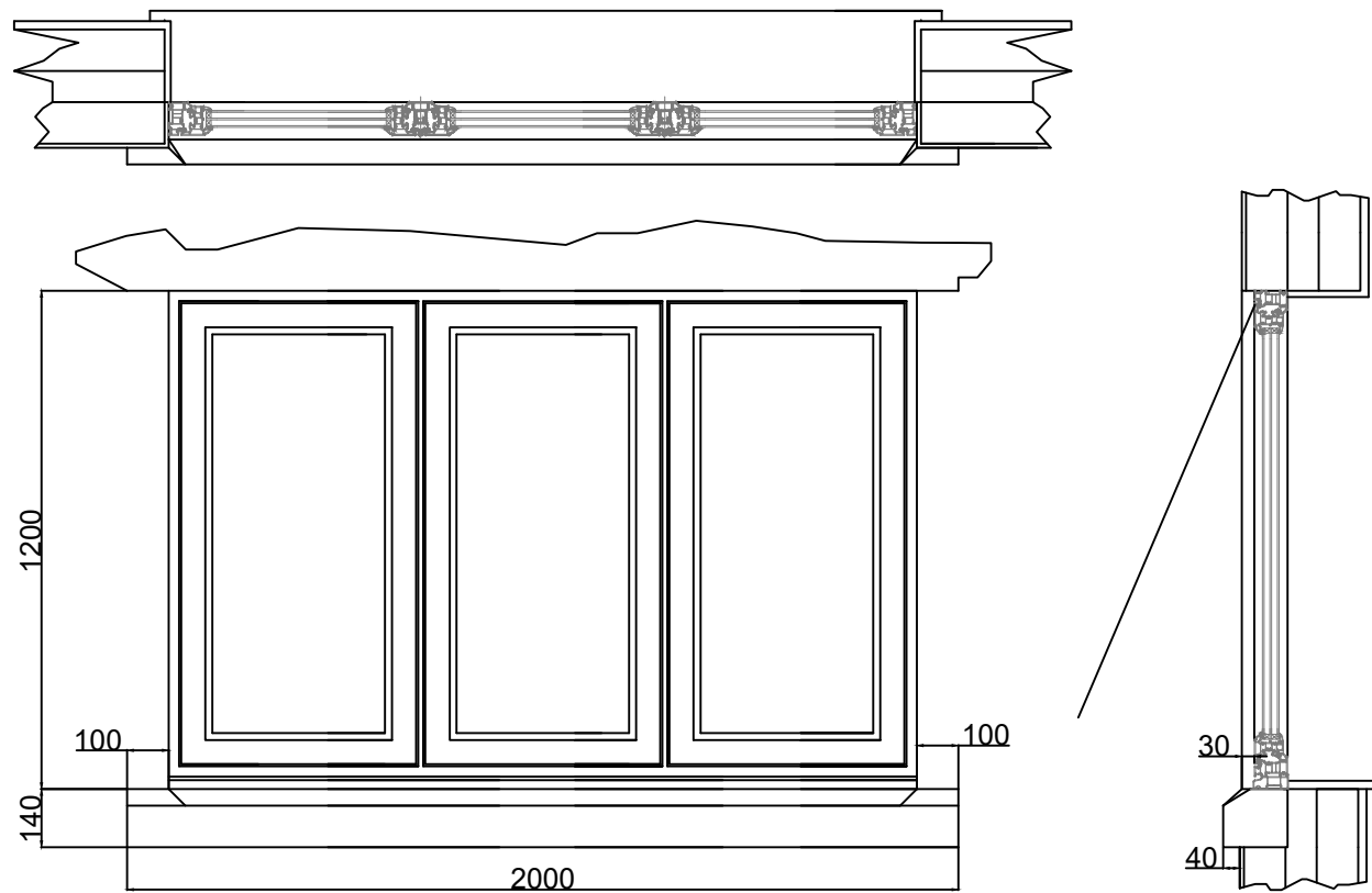
Window: Rear, first floor, left en-suite, obscured glass, Scale 1 / 20
