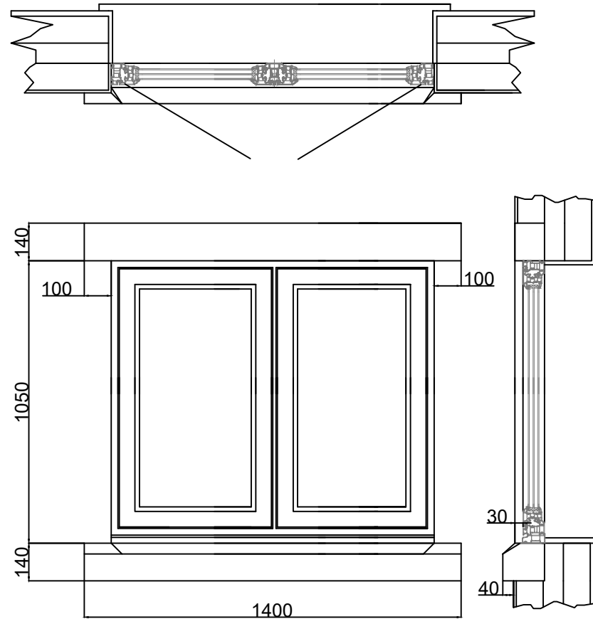
Window: Rear, ground floor, Left bedroom, clear glass, Scale 1 / 20
