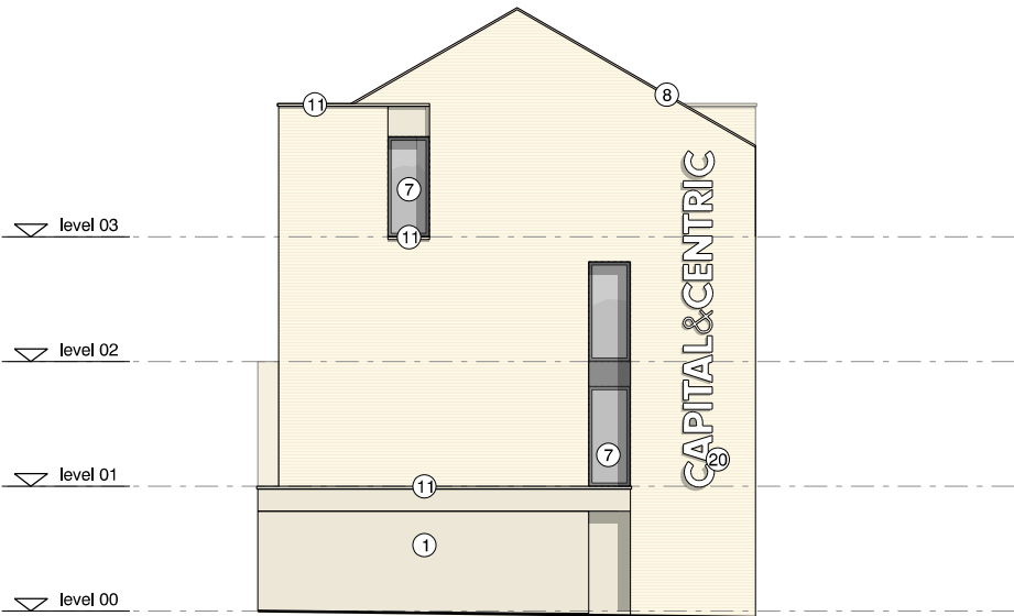
elevation 03 (new wye street)
