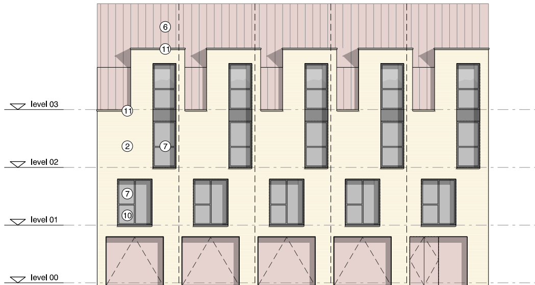
elevation 03
