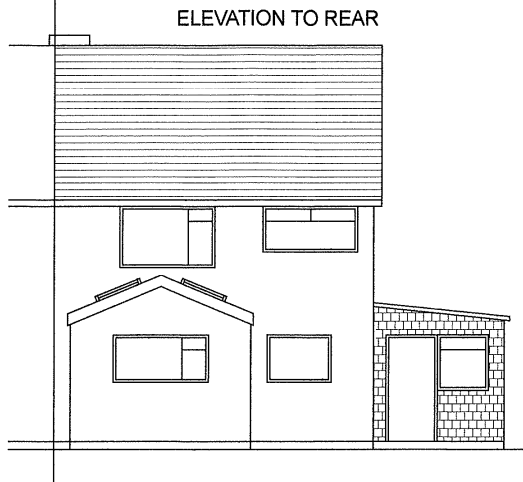
ELEVATION TO REAR
