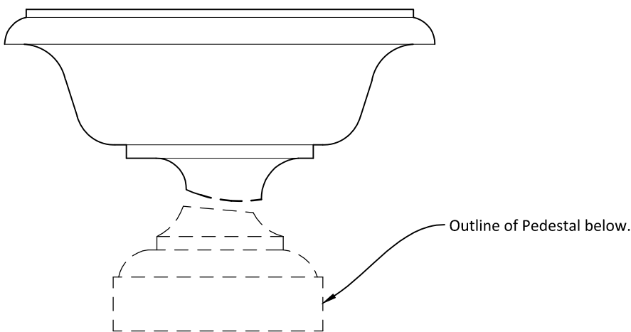
URN ELEVATION (1:10)
