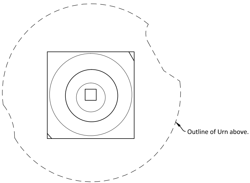
PEDESTAL PLAN (1:10)
