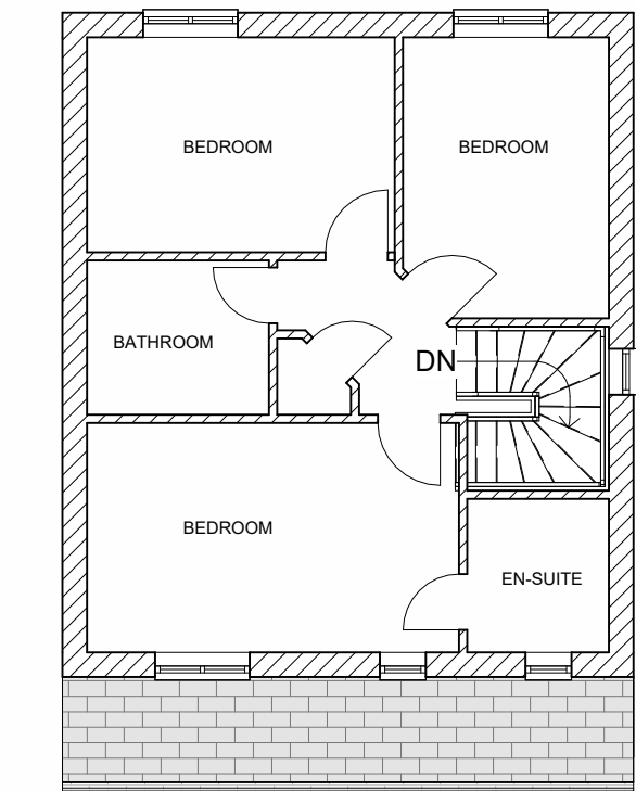
First - proposed 1 : 100
