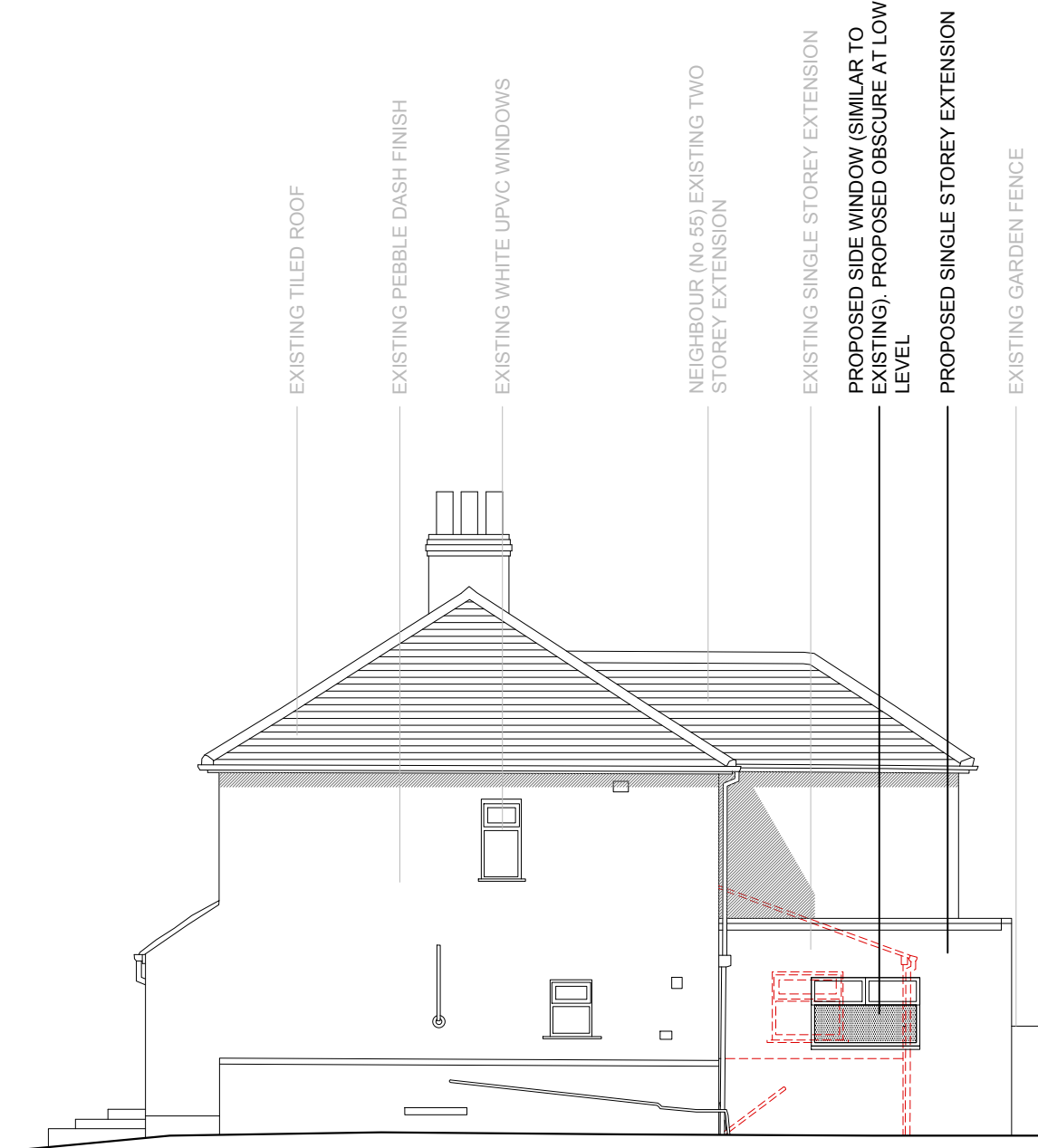
PROPOSED SOUTH (SIDE) ELEVATION - 1:100
