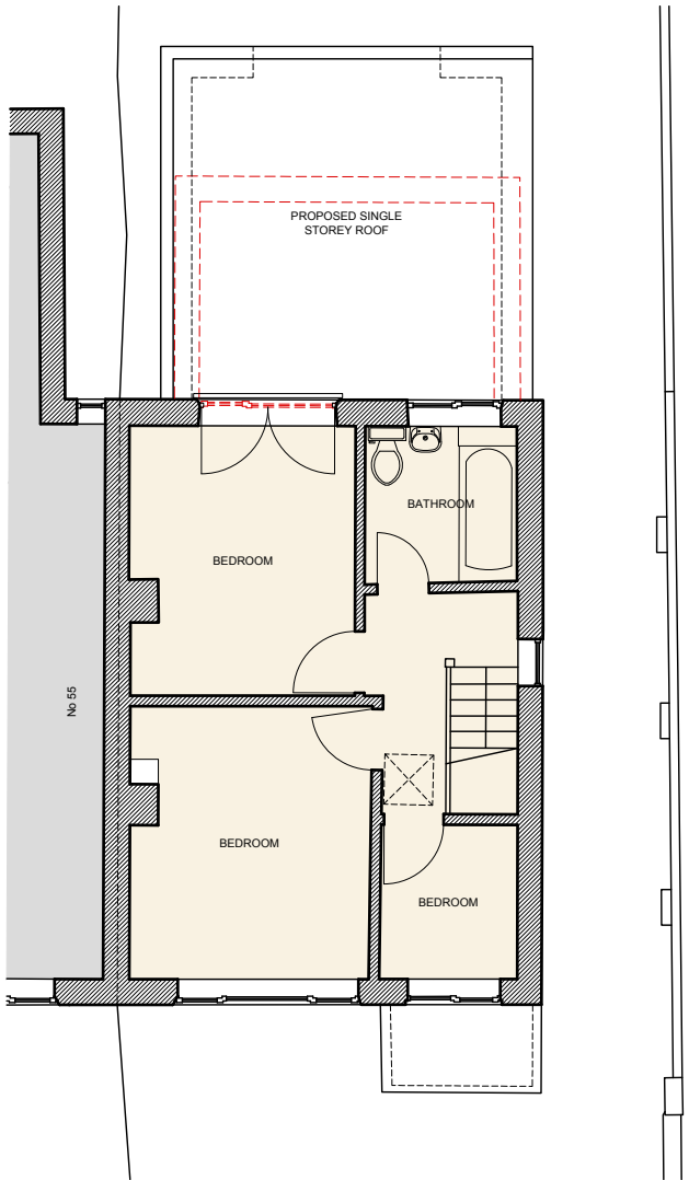
PROPOSED FIRST FLOOR PLAN - 1:100
