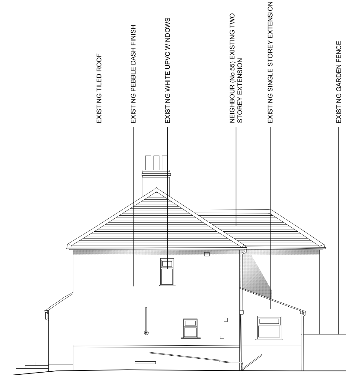
EXISTING SOUTH (SIDE) ELEVATION - 1:100
