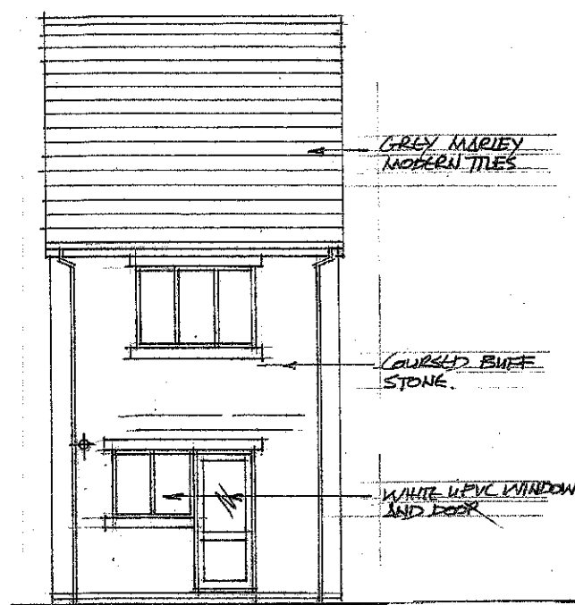
REAR ELEVATION WEST
