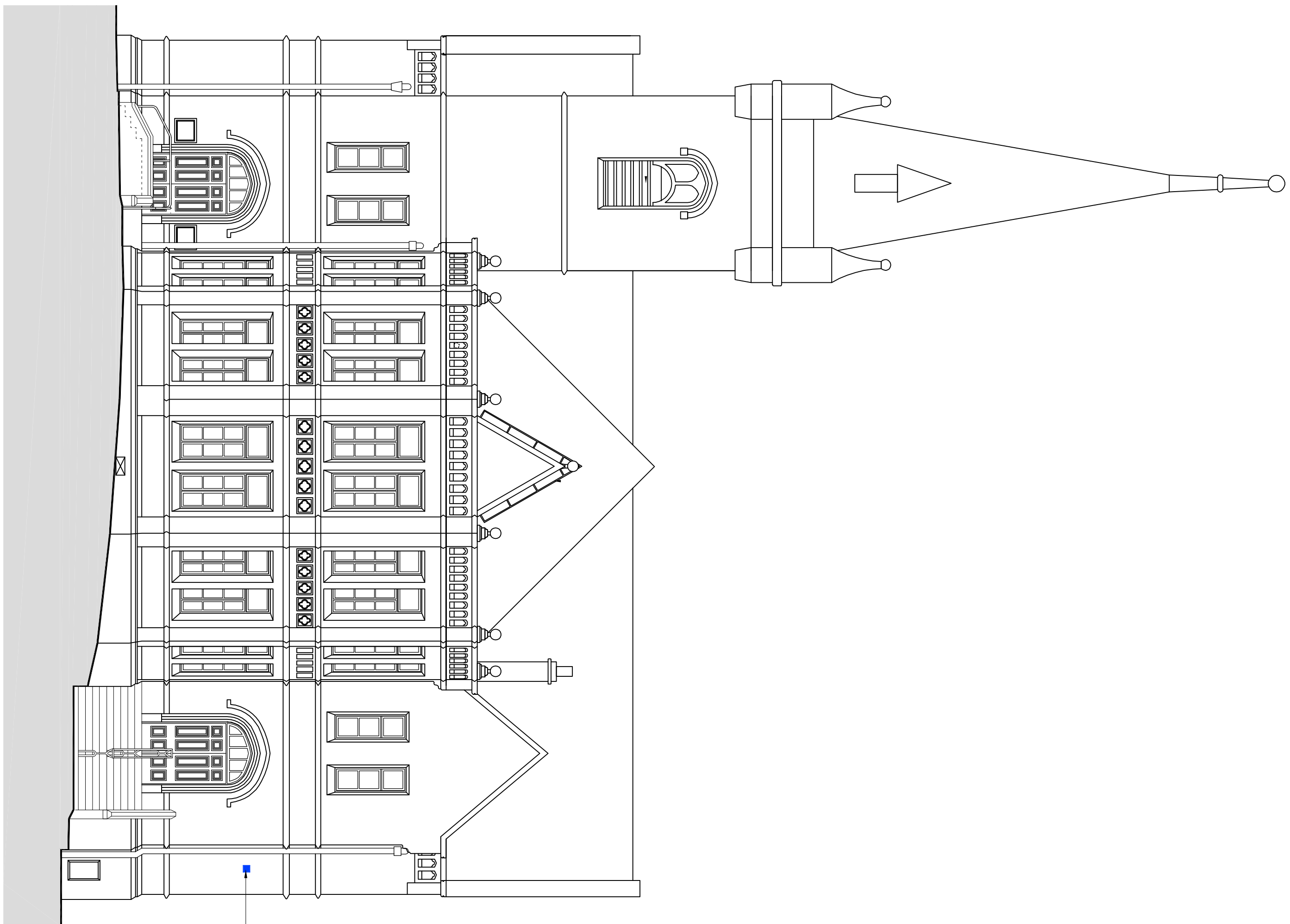
Proposed Elevation A
