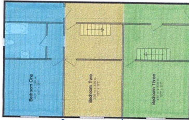
Lower Ground
