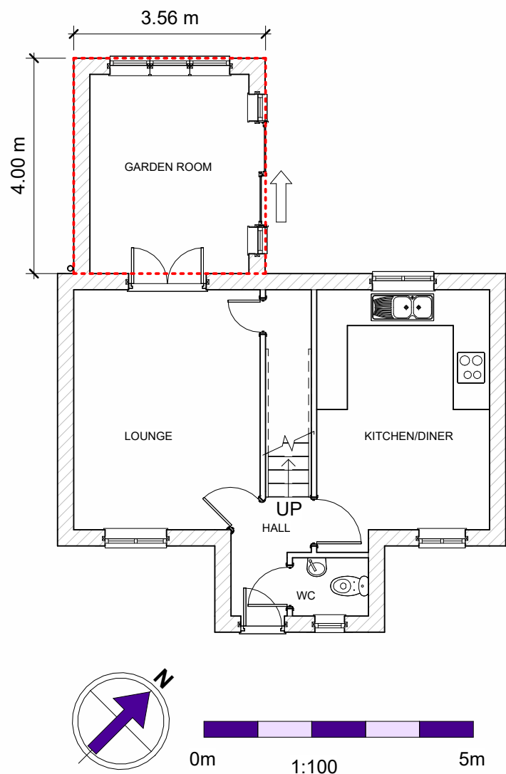
Ground Proposed 1 : 100
