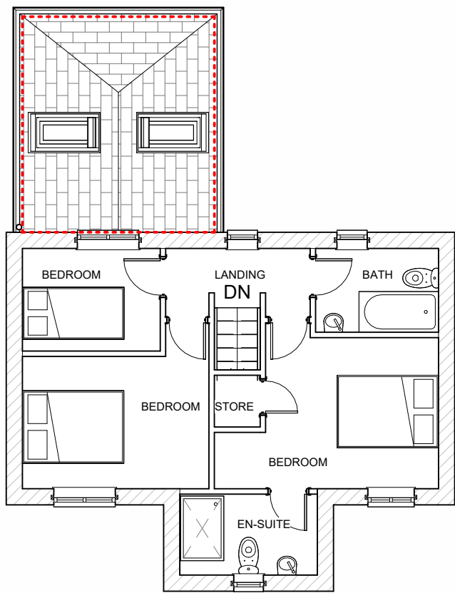
First Proposed 1 : 100
