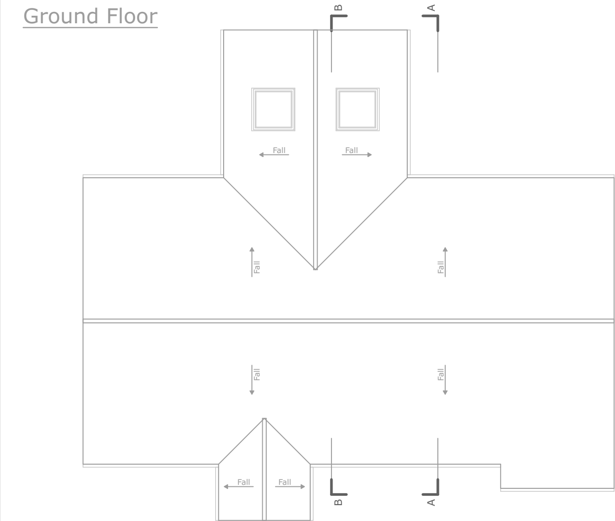
Roof Plan
