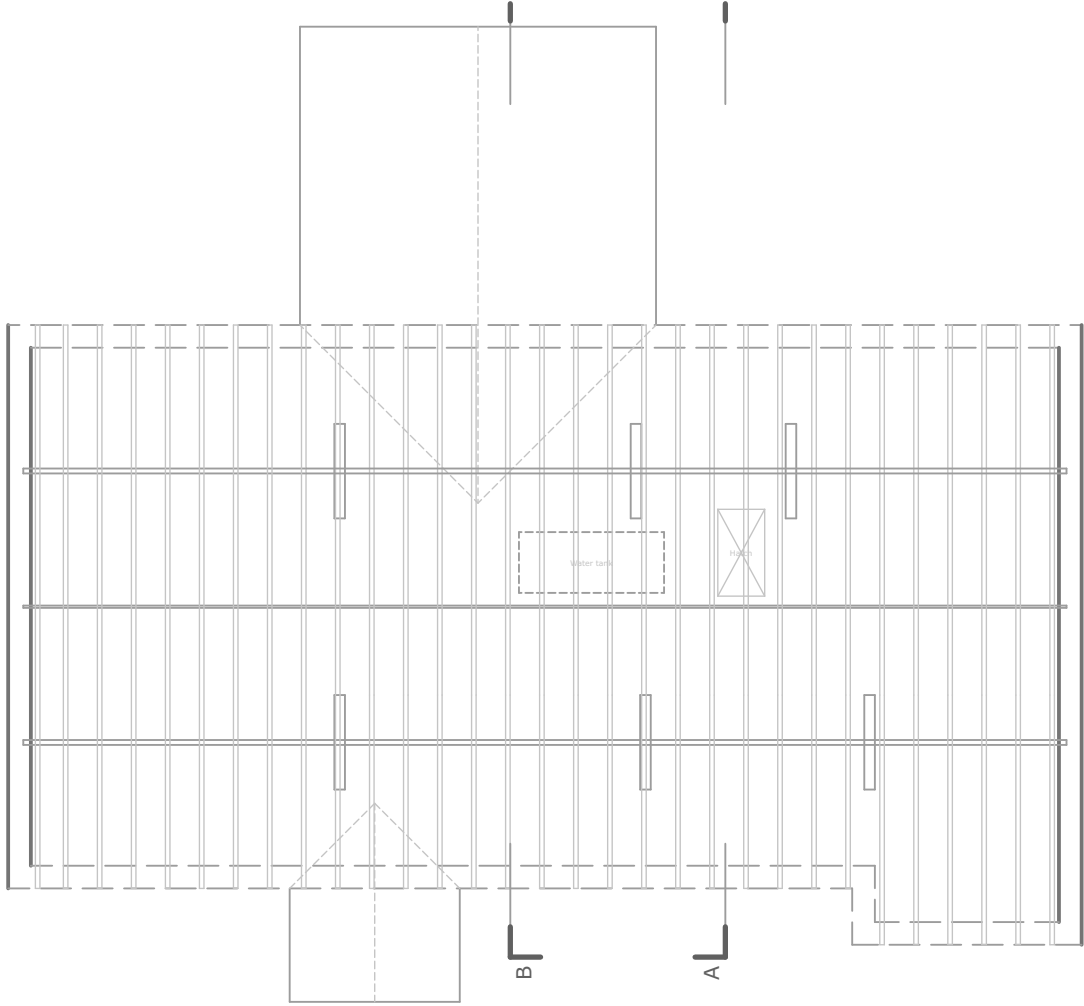
First Floor
