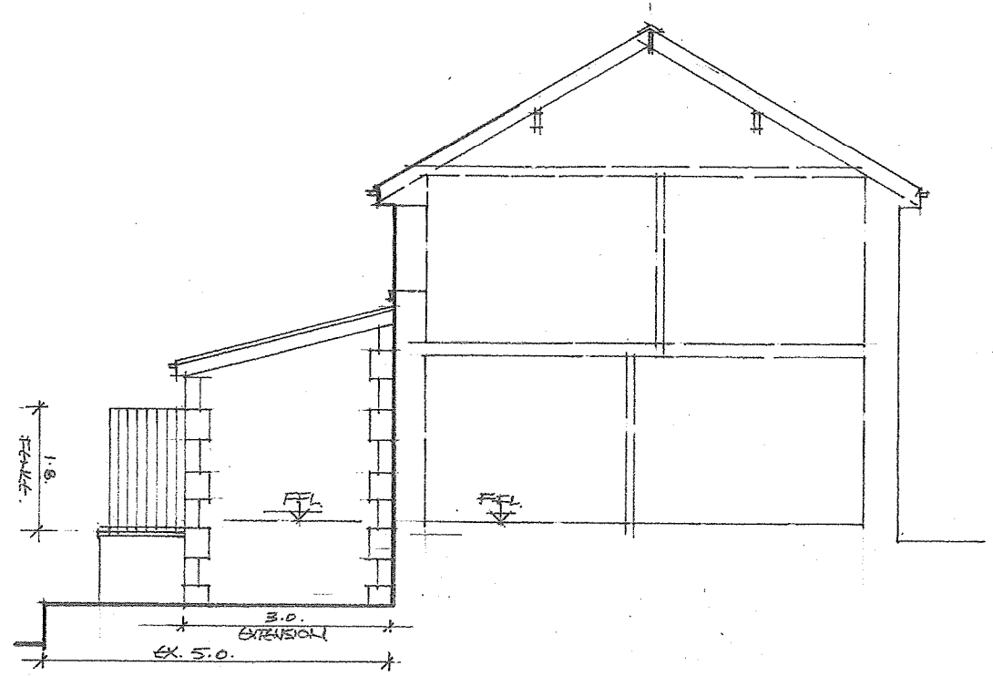
SIDE ELEVATION S.W.
