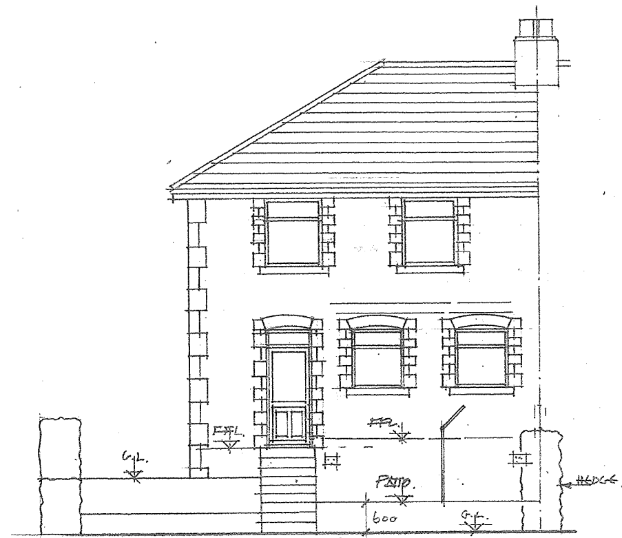
REAR ELEVATION N.W.
