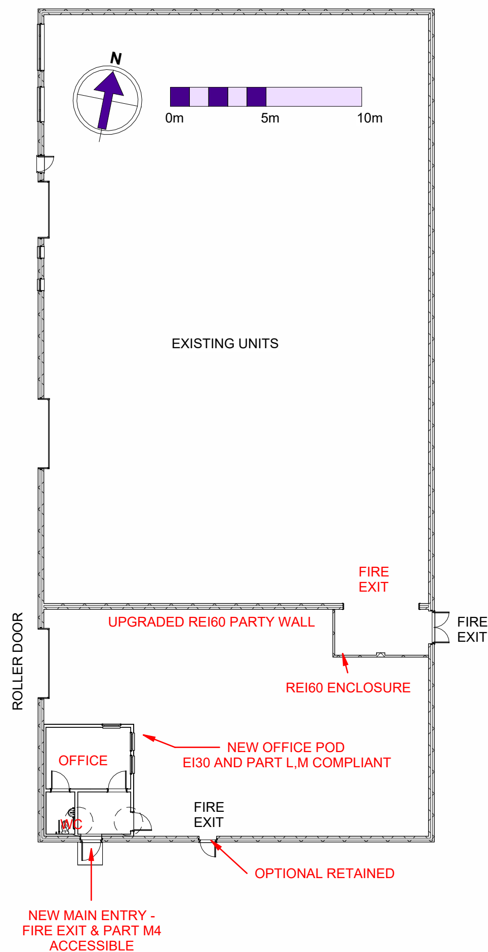
00 GROUND Proposed 1 : 200
