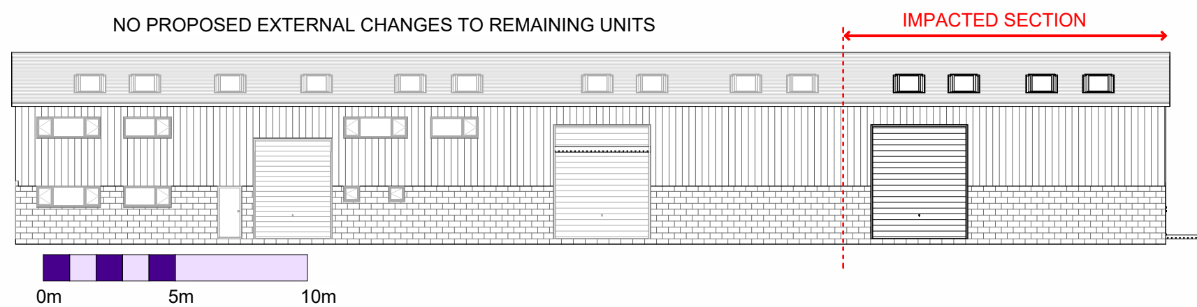
Front (W) - Proposed
