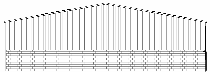
Side (N) - Proposed
