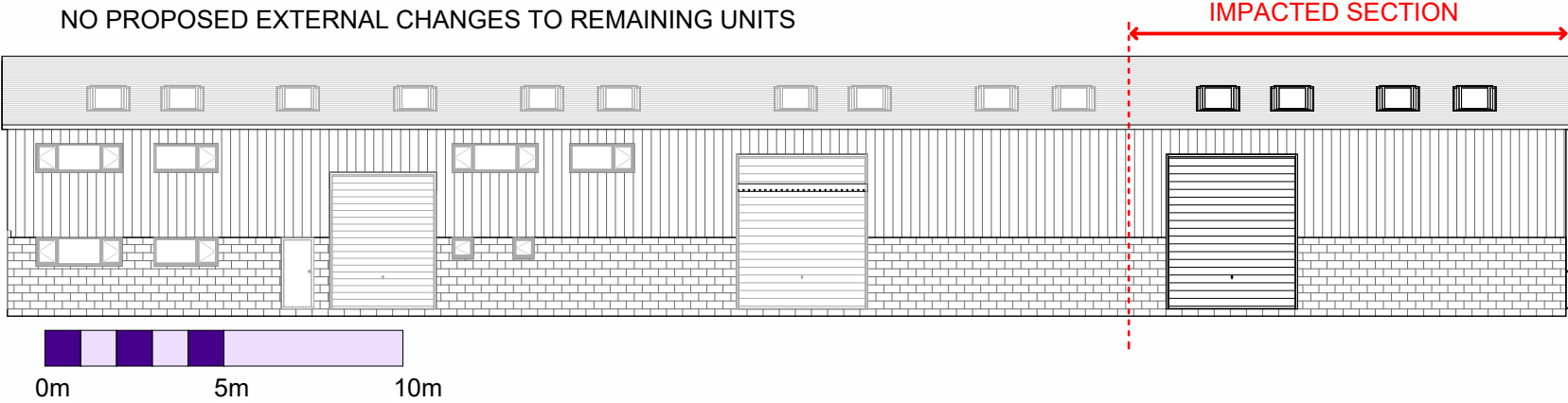
Front (W) - Existing 1 : 200
