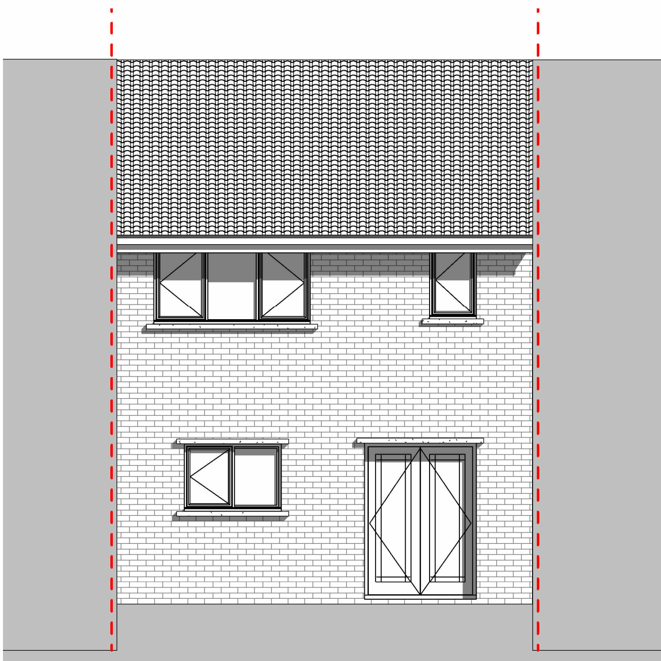
Rear Elevation 1 : 50
