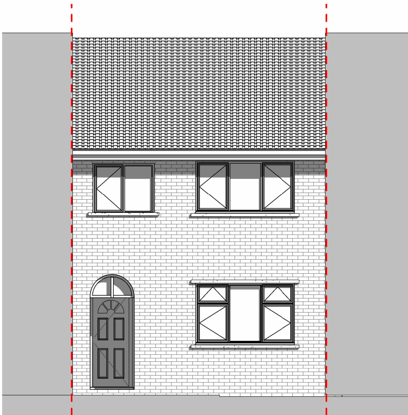
Front Elevation 1 : 50
