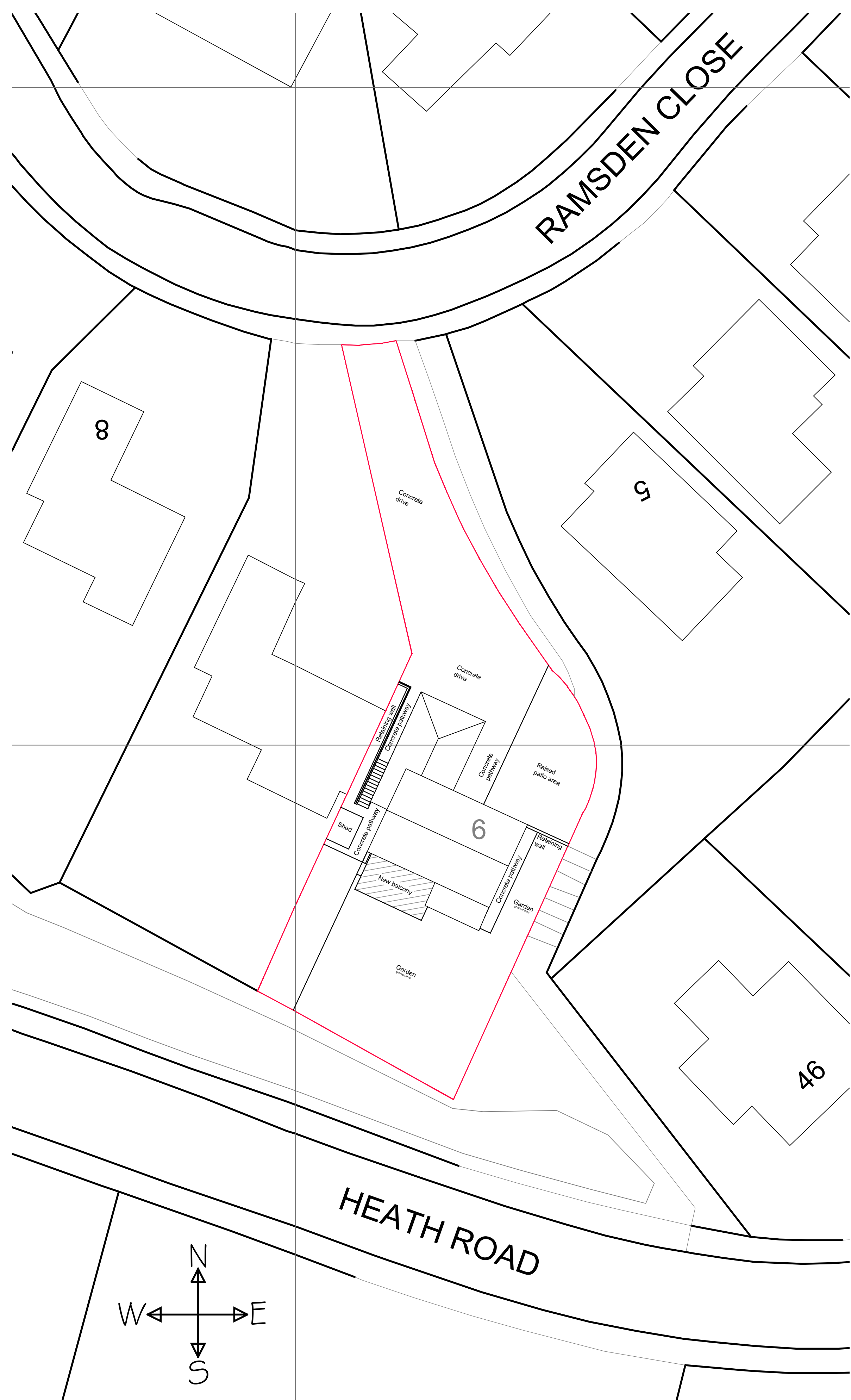
Proposed Site Layout Scale 1:200
