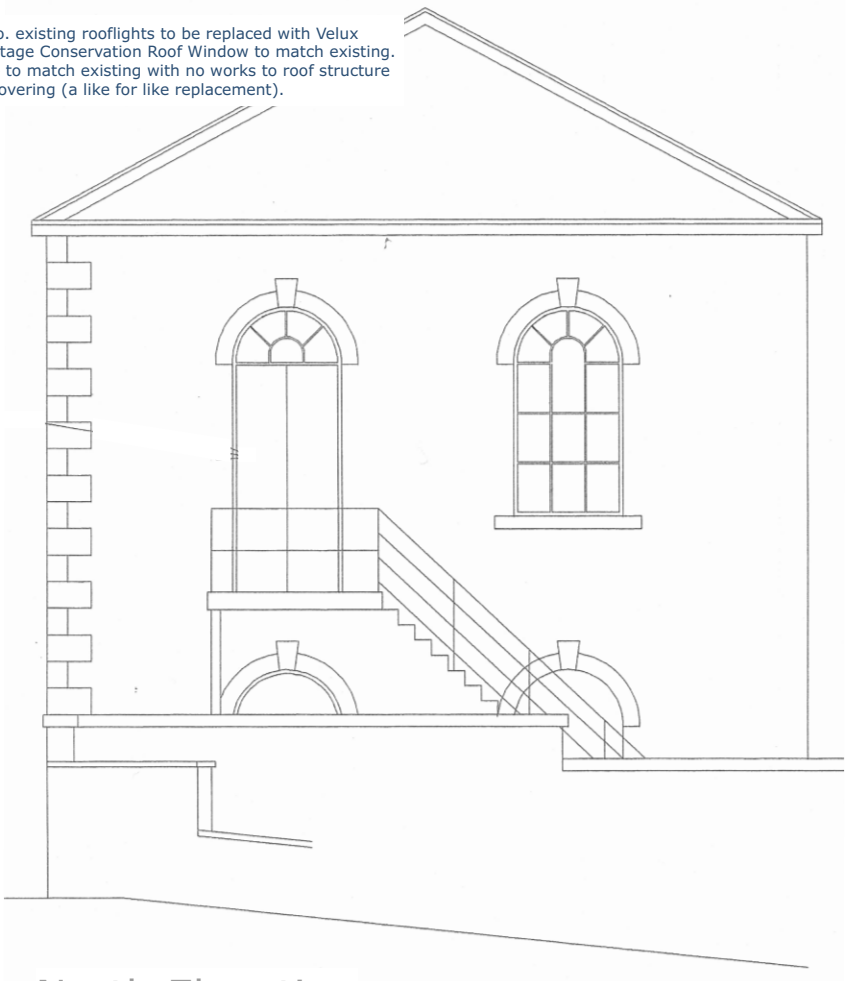
North Elevation
