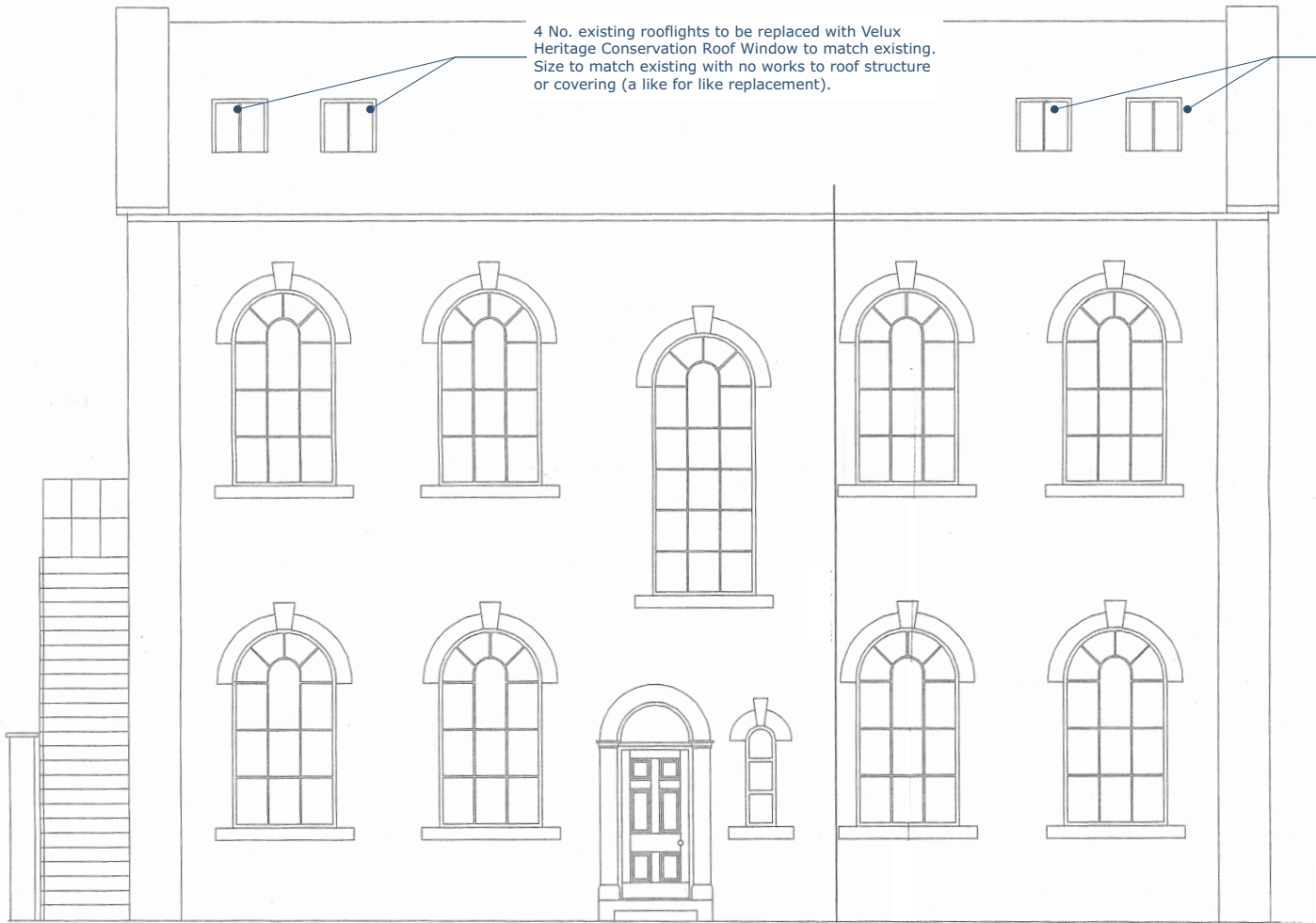
West Elevation
