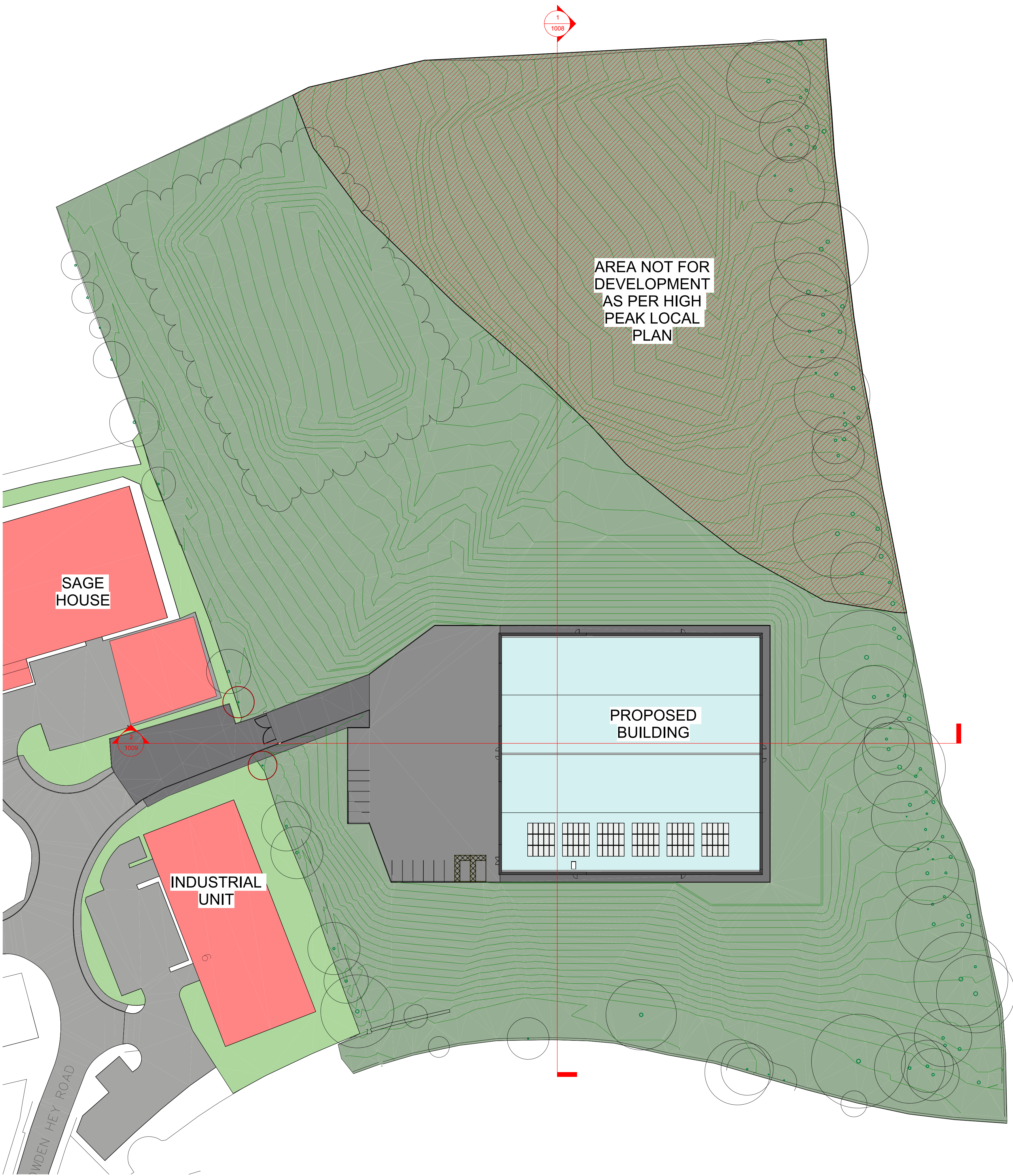
Site Block Plan Proposed 1 : 500
