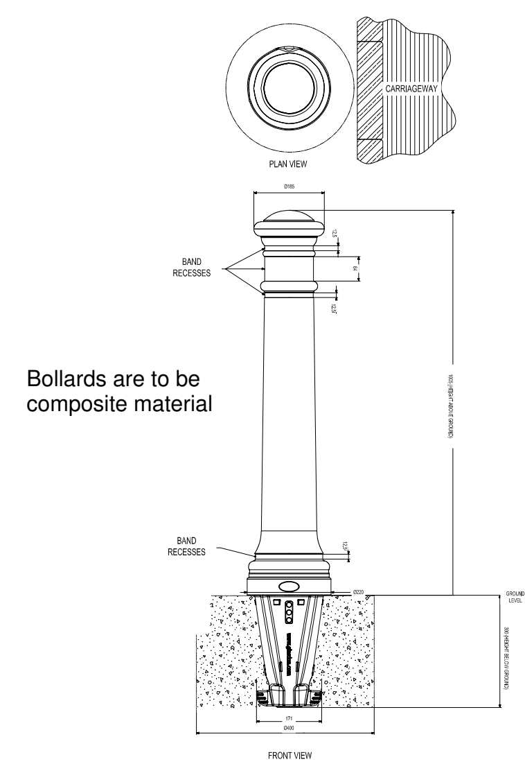
BOLLARD DETAIL SCALE - 1:20
