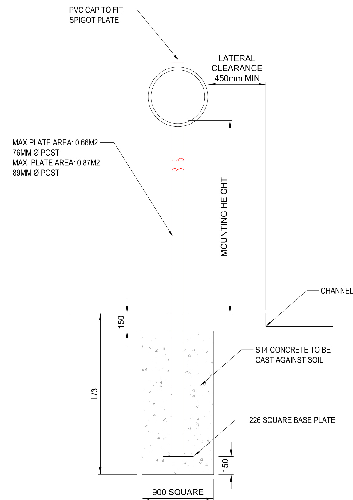
MOUNTING SIGN DETAIL SCALE - 1:20
