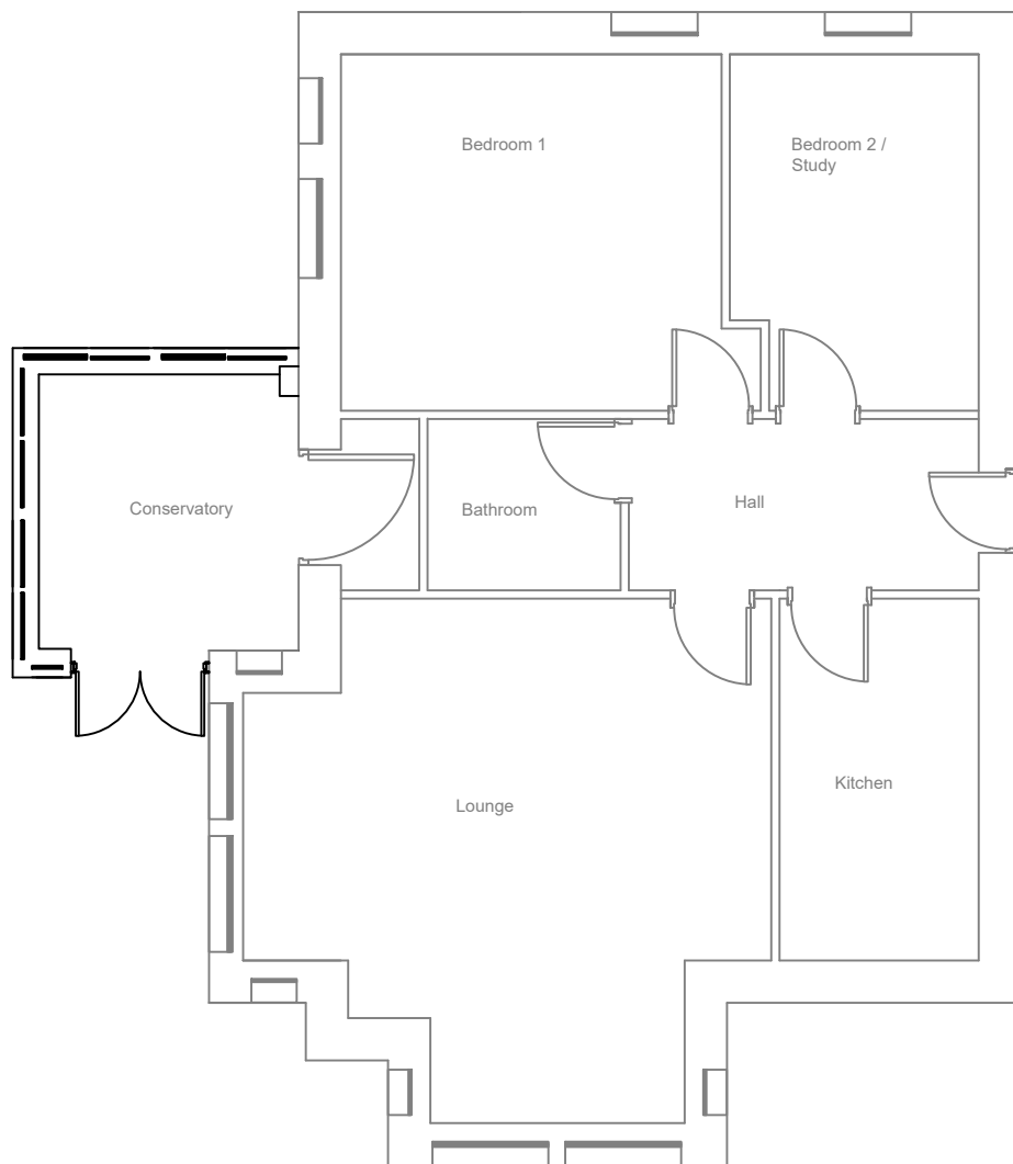
Application No PP-13421709 Proposed new conservatory and flat plan. Drawing Date 23/5/25 Scale 1:100 @ A4
