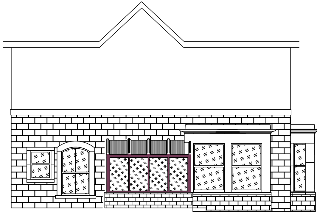
Application No PP-13421709 Existing conservatory side elevation (v2) Drawing Date 23/5/25 Scale 1:100 @ A4
