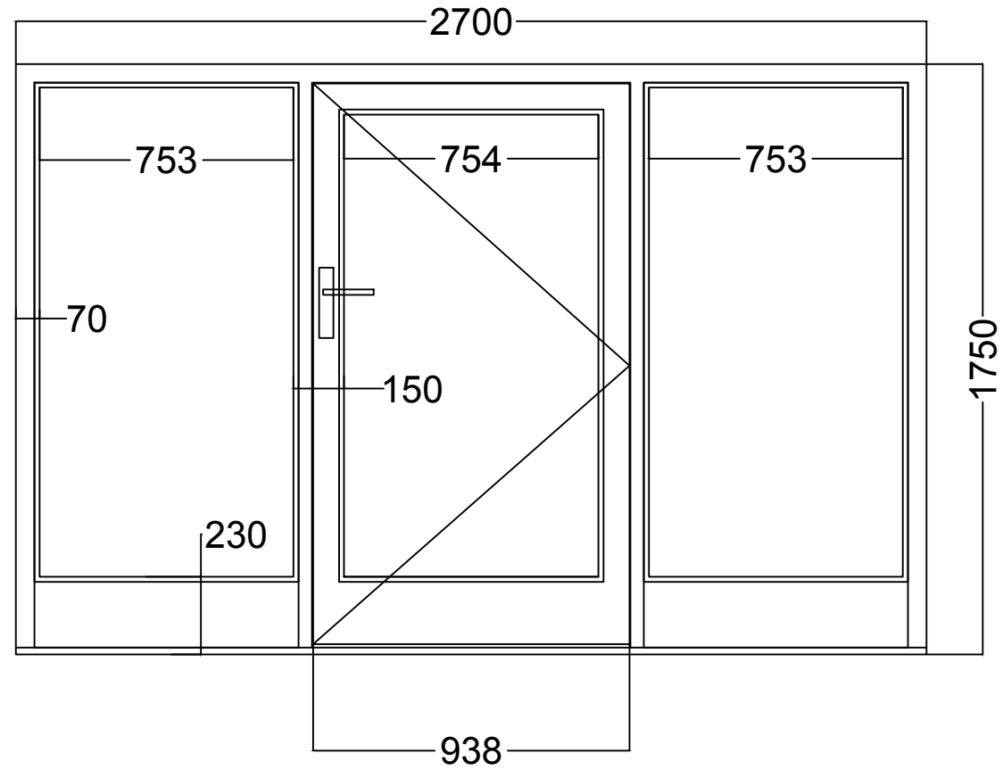
Proposed adaptation to existing opening. Bottom rail run through to give chip protection at floor level. Minimal top rail to maximise light. Glass areas currently equidistant but can be set to accommodate furniture or wheelchair access.
