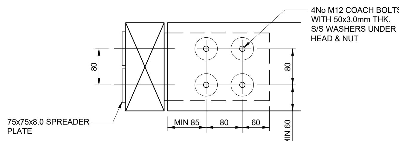
ELEVATION ON JOINTS SCALE 1:5
