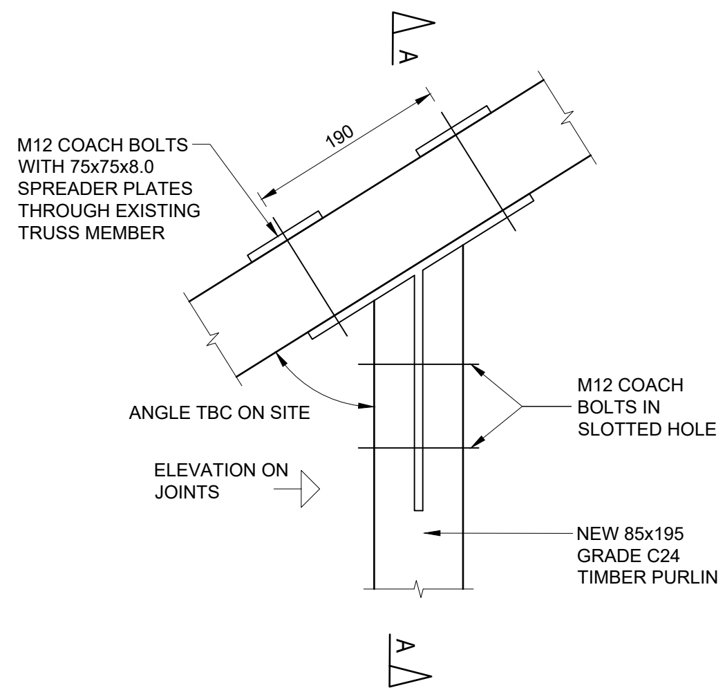
PLAN ON DETAIL A/C - FLITCH TEE JOINT SCALE 1:5
