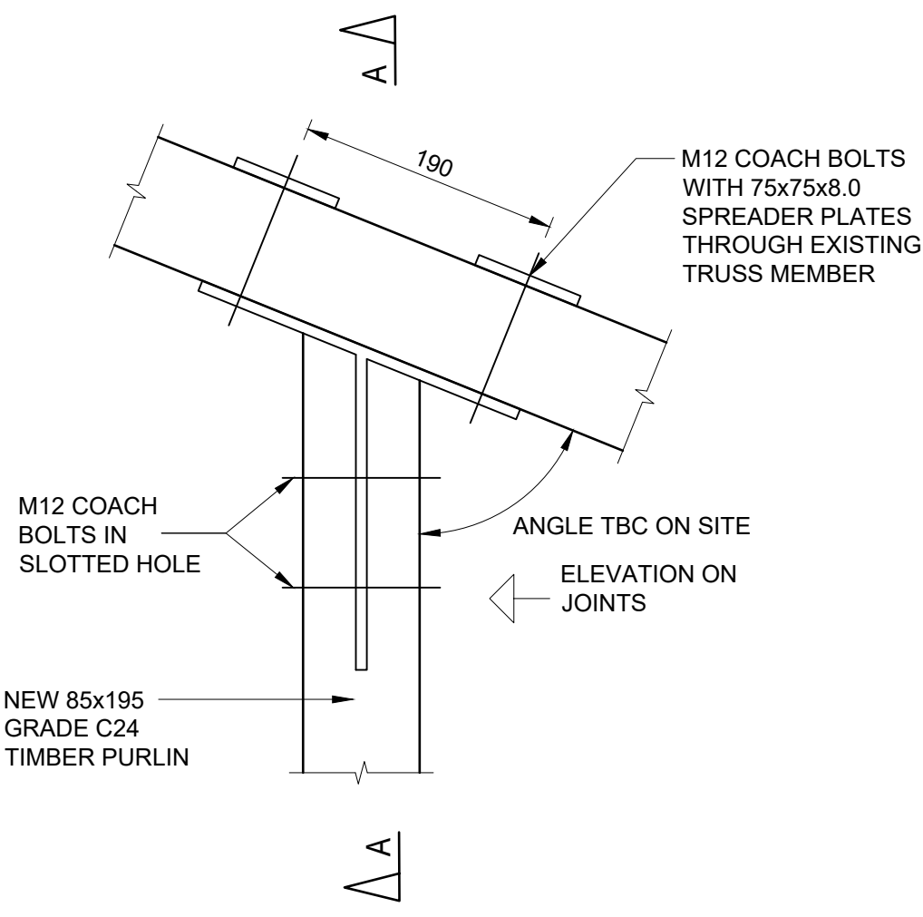
PLAN ON DETAIL B/D - FLITCH TEE JOINT SCALE 1:5
