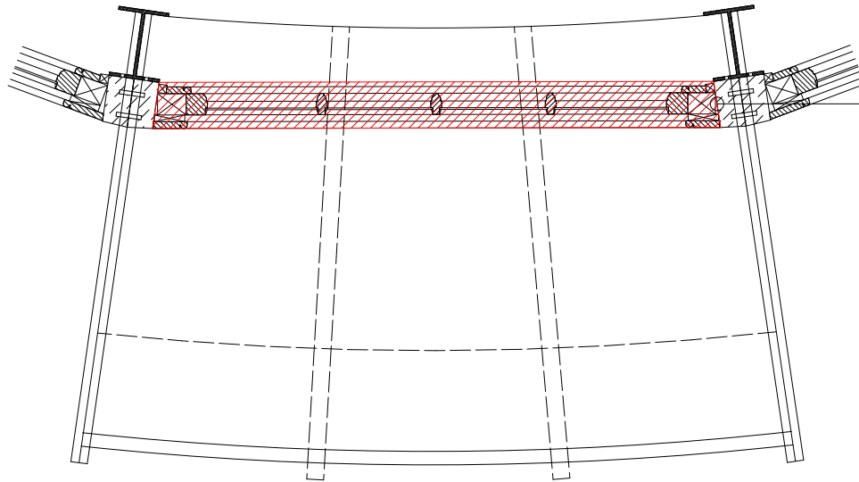
PLAN LAYOUT OF TYPICAL BAY MODULE 1:20
