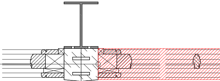
PLAN DETAIL JUNCTION AT TYPICAL BAY MODULE 1:10
