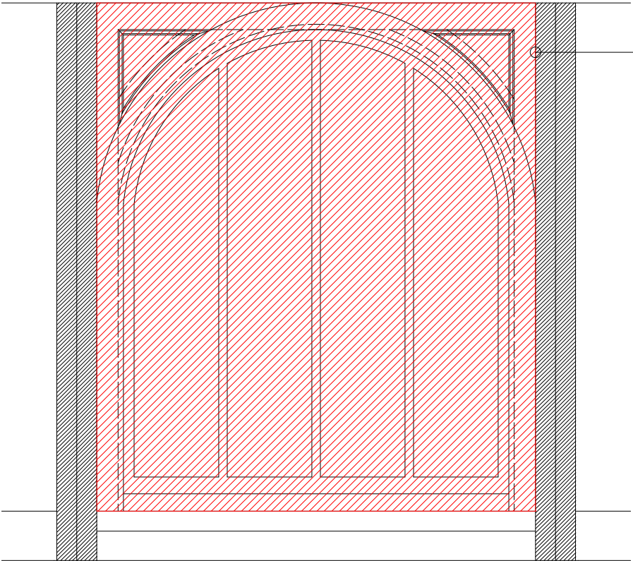
WINDOW MODULE ELEVATION 1:20
