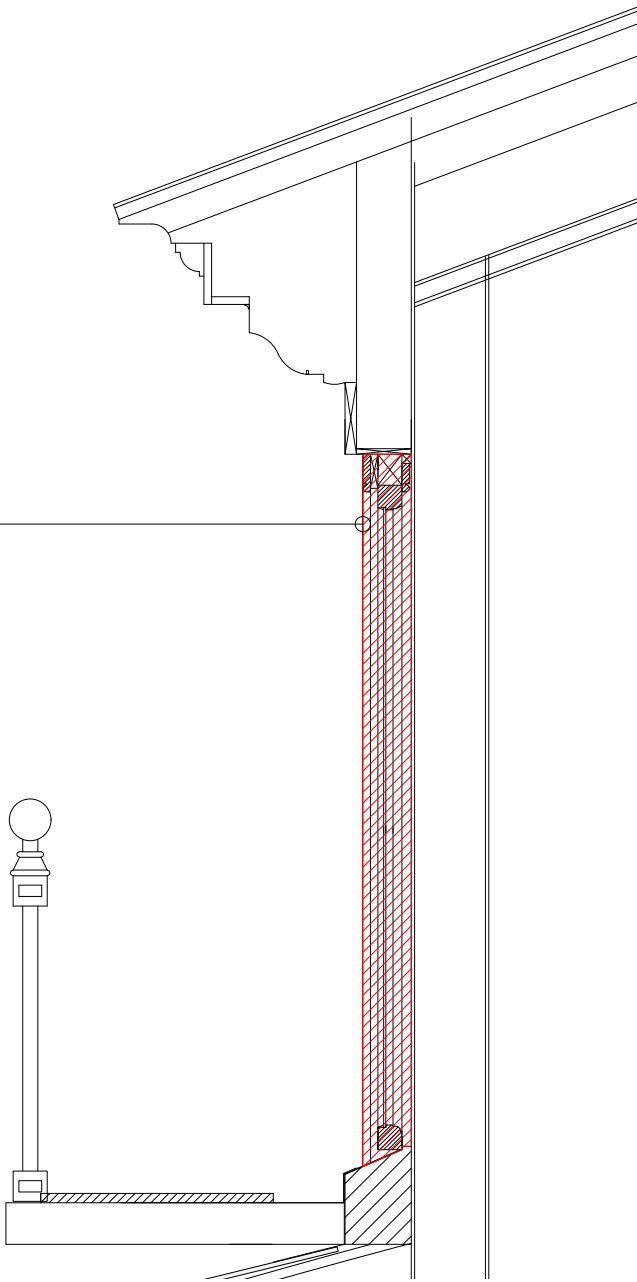
WINDOW MODULE SECTION 1:20
