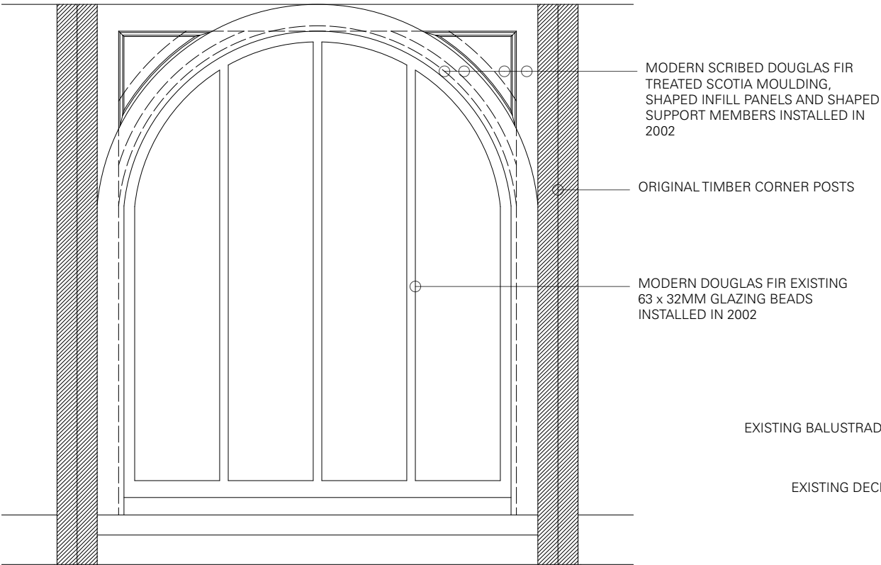
WINDOW MODULE ELEVATION 1:20
