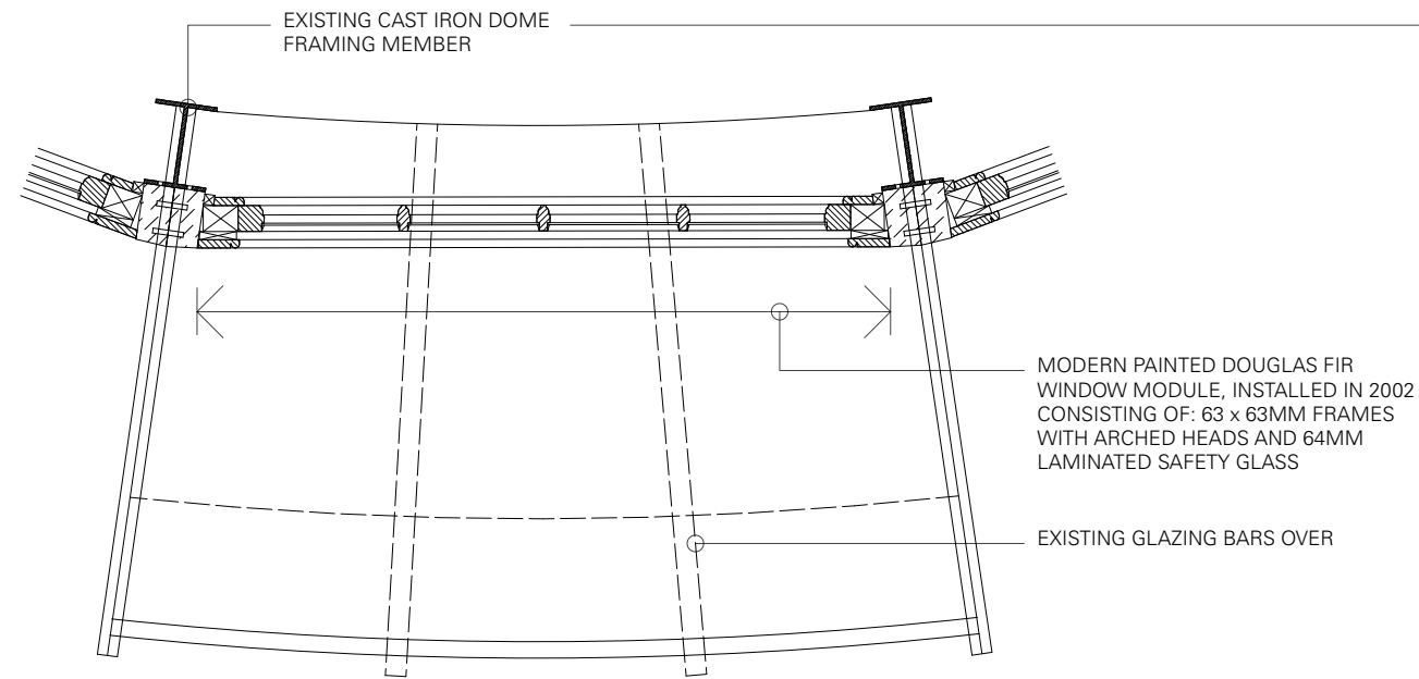
PLAN LAYOUT OF TYPICAL BAY MODULE 1:20
