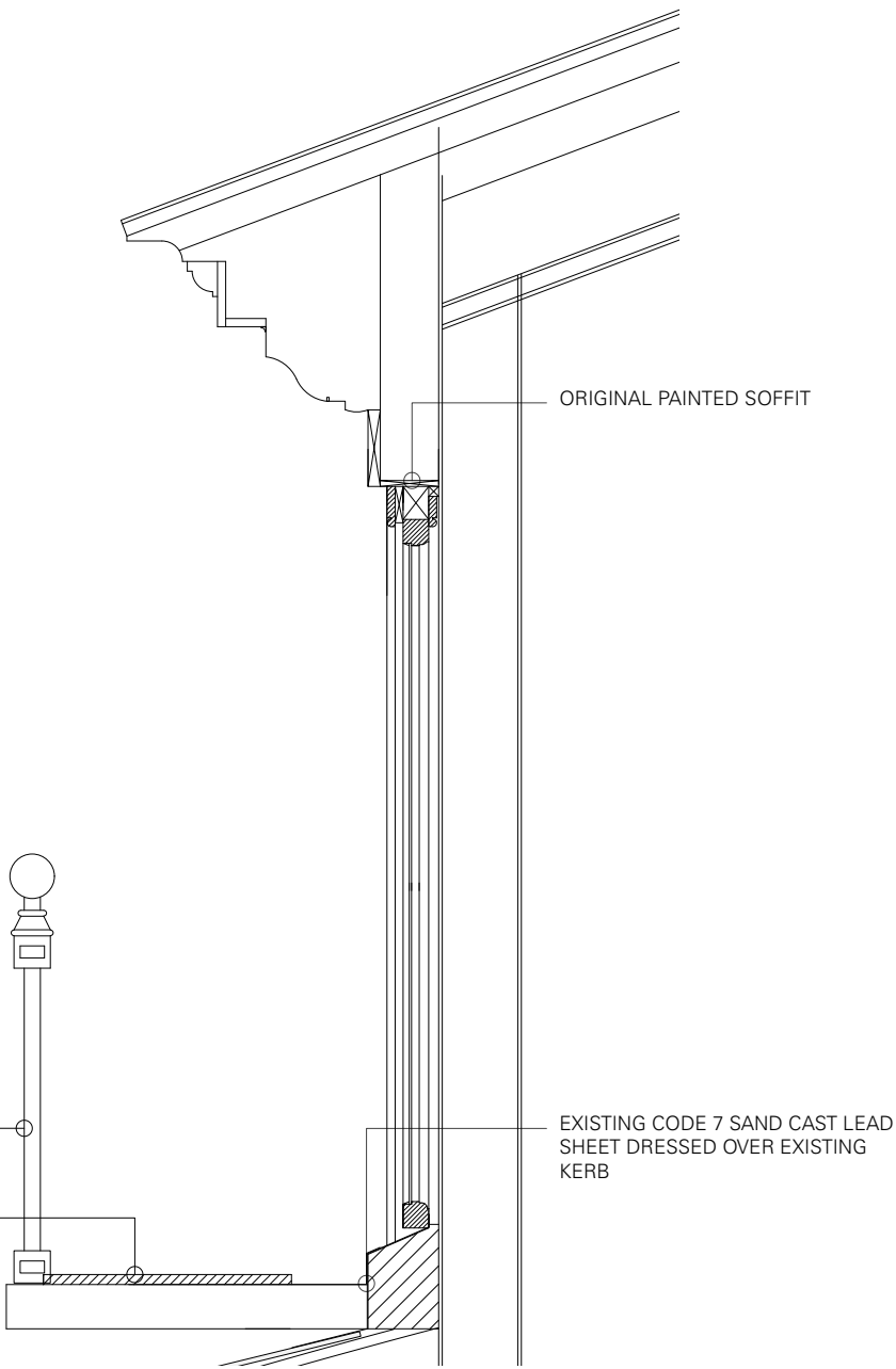
WINDOW MODULE SECTION 1:20
