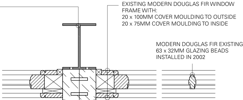
PLAN DETAIL JUNCTION AT TYPICAL BAY MODULE 1:10
