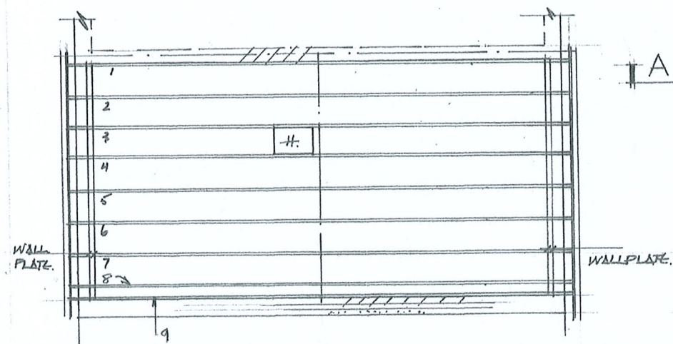
LOFT PLAN 9 No TRUSSES
