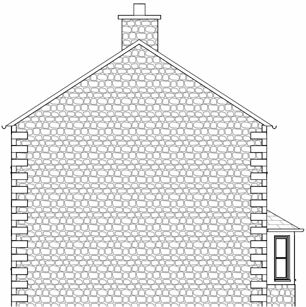
Side - North 1 : 100
