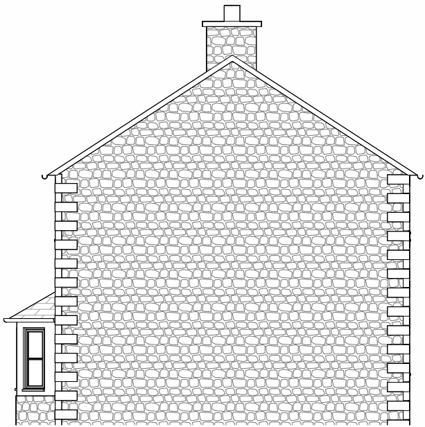
Side - South 1 : 100
