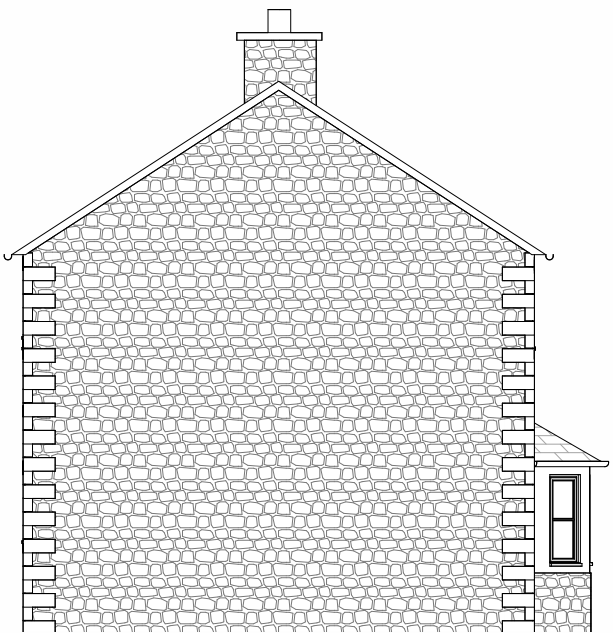
Side - North 1 : 100
