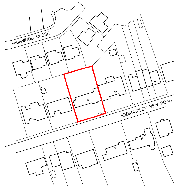
LOCATION PLAN - 1:1250
