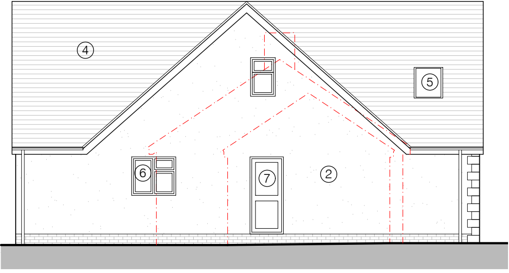
WEST ELEVATION - 1:100
