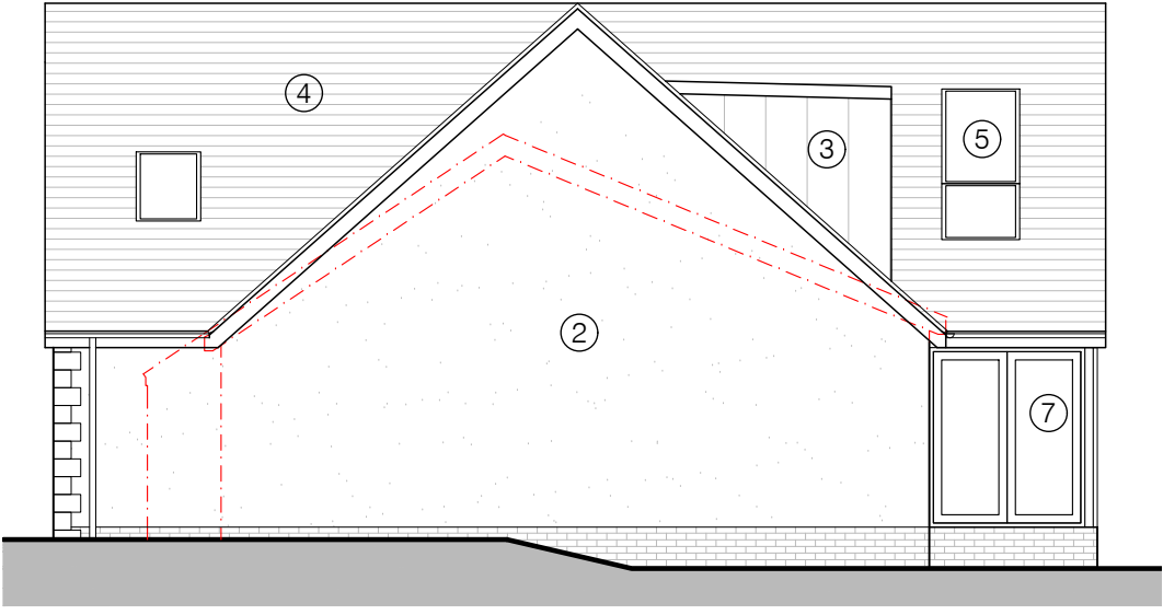
EAST ELEVATION - 1:100
