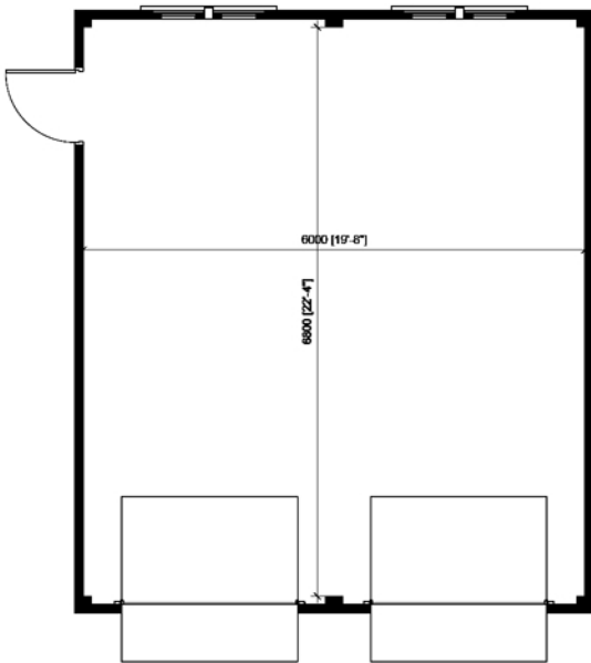
floor plan
