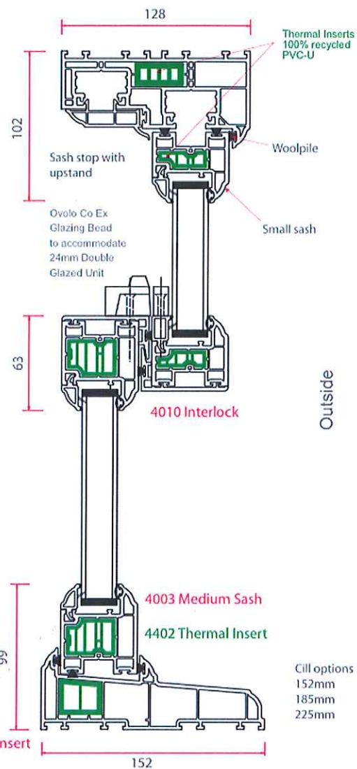
Vertical section through top sash
