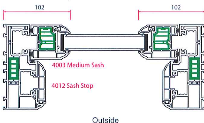
Horizontal section through bottom sash
