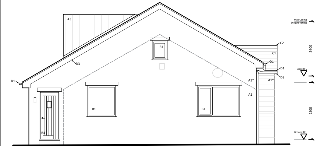
PROPOSED SOUTH EAST ELEVATION (GABLE)
