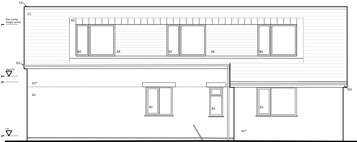
PROPOSED SOUTH WEST ELEVATION (REAR)
