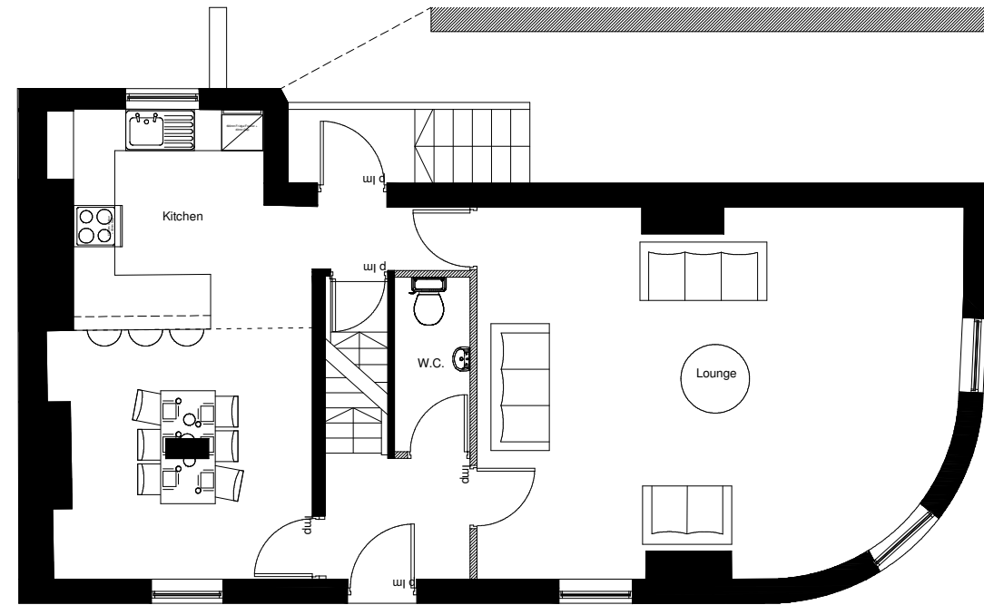
2 Proposed Ground Floor Plan 1 : 100
