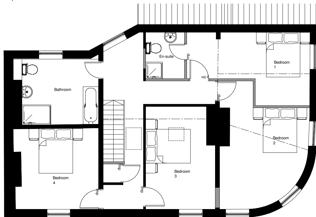
3 Proposed First Floor Plan 1 : 100
