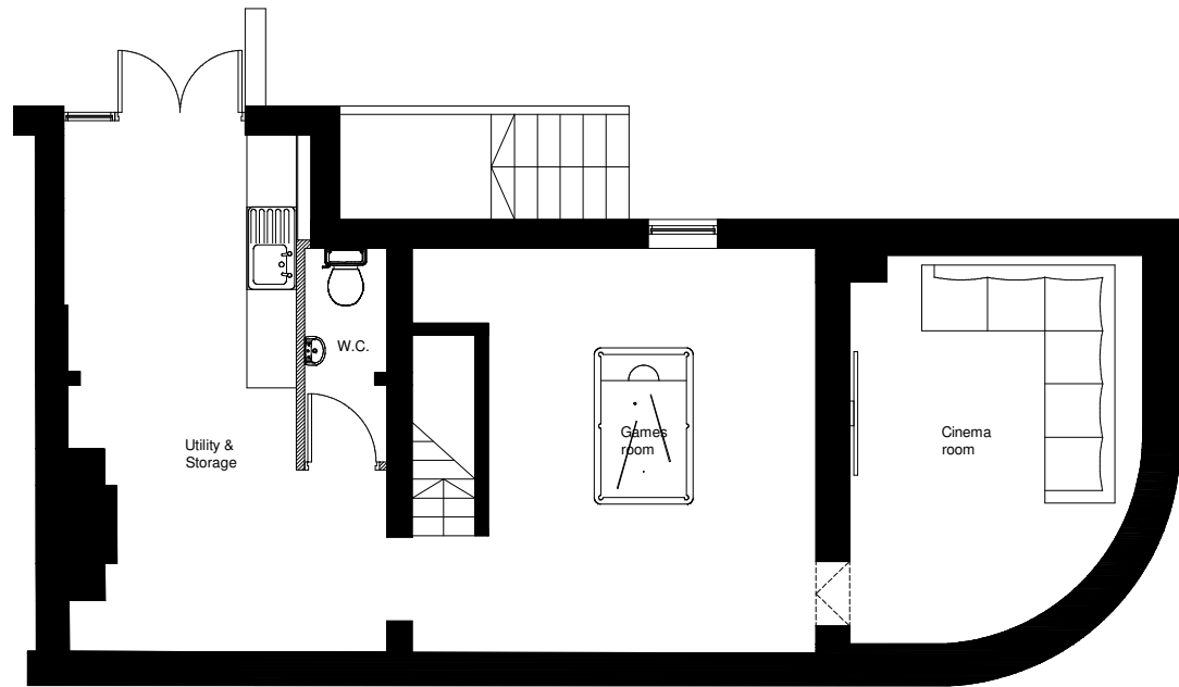
1 Proposed Basement Floor Plan 1 : 100
